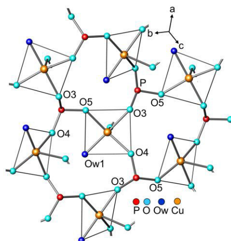
Figure 17. Connections between adjacent \text{Cu}^{2+} coordination polyhedra in \text{Cu}[(\text{RS})\text{-}\mu_3\text{-O}_3\text{PCH}(\text{C}_2\text{H}_5)\text{COOH}]\cdot 3\text{H}_2\text{O} ( 2 ). Carbon, hydrogen and oxygen atoms not bond to \text{Cu}^{2+} are omitted for clarity. Thin black lines illustrate the equatorial planes.
