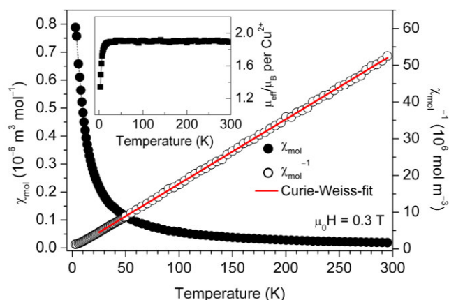
Figure 15. Susceptibility versus temperature of \text{Cu}[(\text{RS})\text{-}\mu_3\text{-O}_3\text{PCH}(\text{C}_2\text{H}_5)\text{COOH}]\cdot 3\text{H}_2\text{O} ( 2 ). The inset shows the temperature development of the magnetic moment in consideration of the Weiss temperature.
