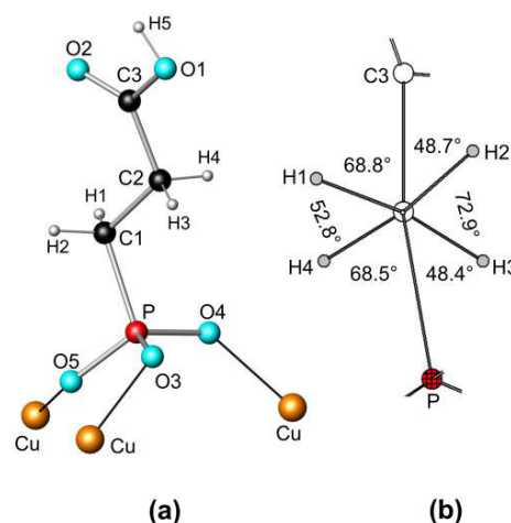
Figure 2. (a) The connection between the dianion of the 3-phosphonopropionic acid and the Cu 2+ cations in Cu[μ 3 -O 3 P(CH 2 ) 2 COOH]·2H 2 O ( 1 ). (b) Newman projection of the [O 3 P(CH 2 ) 2 COOH] 2- dianion along C(1)–C(2).
