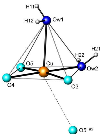
Figure 1. The square pyramidal coordination (thick black bonds) of Cu 2+ in Cu[μ 3 -O 3 P(CH 2 ) 2 COOH]·2H 2 O ( 1 ). The index (#) indicates the longest Cu–O distance. Symmetry code #2: x-0.5; -y+1.5; -z+1.
