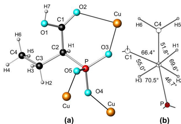
Figure 7. (a) The connection between the [O 3 PCH(C 2 H 5 )COOH] 2- dianion and the copper cations in 2. (b) Newman projection of the [O 3 PCH(C 2 H 5 )COOH] 2- dianion along C(2)–C(3). The figures show the S enantiomer.
