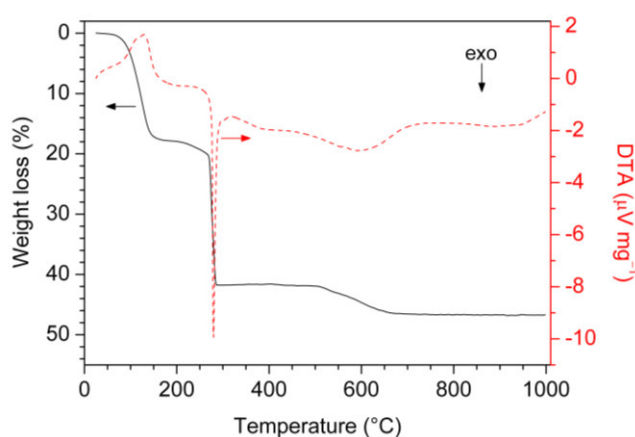
Figure 12. Thermal analysis of \text{Cu}[(\text{RS})\text{-}\mu_3\text{-O}_3\text{PCH}(\text{C}_2\text{H}_5)\text{COOH}]\cdot 3\text{H}_2\text{O} ( 2 ).
