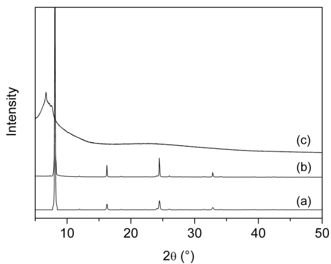
Figure S3. X-ray powder diffraction patterns of \text{Cu}[(\text{RS})\text{-}\mu_3\text{-O}_3\text{PCH}(\text{C}_2\text{H}_5)\text{COOH}]\cdot 3\text{H}_2\text{O} ( 2 ). (a) calculated pattern, (b) experimental pattern, c) pattern after heating at 200 °C. The pattern of graph (a) was calculated using the March-Dollase model with a (001) preferred orientation.
