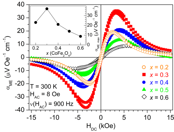
Fig. 12: Magnetoelectric coefficient ( \alpha_{ME} ) vs. magnetic DC field for various composite ceramics sintered at 1100 °C for 1 h. The inset shows the maximum magnetoelectric coefficient ( \alpha_{ME,max} ) depending on the CoFe_2O_4 fraction ( x ). The uncertainty of the data ( 1 \mu V Oe^{-1} cm^{-1} ) is smaller than the symbol size.
