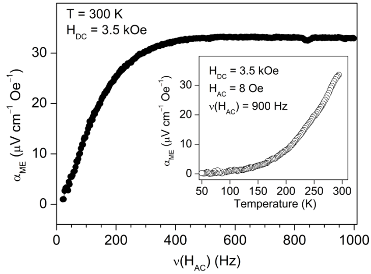
Fig. 14: Frequency dependence ( H_{AC} ) of \alpha_{ME} for (Sr_{0.5}Ba_{0.5}Nb_2O_6)_{0.7}-(CoFe_2O_4)_{0.3} sintered at 1100 °C for 1 h. The inset shows the temperature dependence of \alpha_{ME} .
