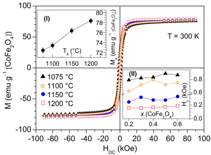
Fig. 7: Magnetization ( M ) versus applied field ( H_{DC} ) at 300 K of (Sr_{0.5}Ba_{0.5}Nb_2O_6)_{0.7}-(CoFe_2O_4)_{0.3} composite bodies sintered at the indicated temperatures for 1 h. Inset (I) shows the saturation magnetization ( M_s ) depending on the sintering temperature ( T_s ). Inset (II) shows the coercivities as a function of the CoFe_2O_4 fraction ( x ) for different sintering temperatures. Uncertainties of the coercivities values ( \leq 20 Oe) are smaller than the symbol sizes. The magnetization is given with respect to the nominal CoFe_2O_4 mass.
