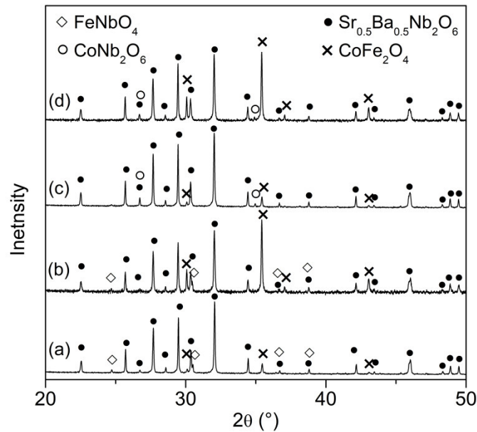
Fig. 5: Room-temperature powder XRD patterns of crushed (\text{Sr}_{0.5}\text{Ba}_{0.5}\text{Nb}_2\text{O}_6)_{1-x}\text{--}(\text{CoFe}_2\text{O}_4)_x composite ceramics after sintering at different temperatures ( T_s ) for 1 h (heating-/cooling rate 5 \text{ K min}^{-1} ): a) x = 0.2 , T_s = 1150 \text{ °C} , b) x = 0.6 , T_s = 1150 \text{ °C} , c) x = 0.2 , T_s = 1200 \text{ °C} , d) x = 0.6 , T_s = 1200 \text{ °C} .
