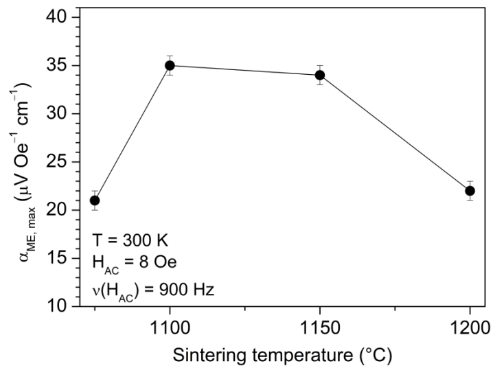
Fig. 13: Maximum magnetoelectric coefficient ( \alpha_{\text{ME,max}} ) depending on the sintering temperature for (\text{Sr}_{0.5}\text{Ba}_{0.5}\text{Nb}_2\text{O}_6)_{0.7}\text{--}(\text{CoFe}_2\text{O}_4)_{0.3} composite ceramics.
