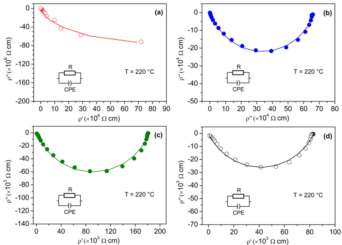
Fig. 11: Cole–Cole plots of (Sr_{0.5}Ba_{0.5}Nb_2O_6)_{1-x}-(CoFe_2O_4)_x ceramics sintered at 1100 °C. a) x = 0.3 , b) x = 0.4 , c) x = 0.5 , d) x = 0.6 .
