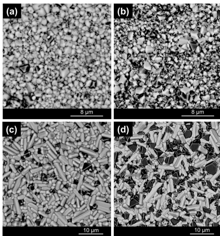
Fig. 4: SEM-BSE images of selected (\text{Sr}_{0.5}\text{Ba}_{0.5}\text{Nb}_2\text{O}_6)_{1-x}\text{--}(\text{CoFe}_2\text{O}_4)_x composite ceramics sintered at different temperatures ( T_s ) for 1 h. (a) x = 0.3 , T_s = 1150 °C, (b) x = 0.6 , T_s = 1150 °C, (c) x = 0.3 , T_s = 1200 °C, (d) x = 0.6 , T_s = 1200 °C.
