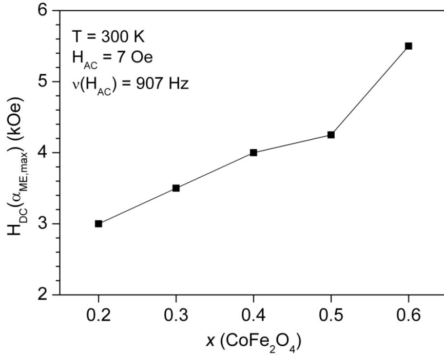
Fig. S6: Magnetic DC field ( H_{\alpha_{\text{max}}} ) at which the magnetoelectric coefficient ( \alpha_{\text{ME,max}} ) reaches its maximum with respect to the \text{CoFe}_2\text{O}_4 fraction ( x ) in (\text{Sr}_{0.5}\text{Ba}_{0.5}\text{Nb}_2\text{O}_6)_{1-x}-(\text{CoFe}_2\text{O}_4)_x composites sintered at 1100 °C for 1 h.
