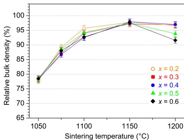
Fig. 3: Relative bulk densities of (\text{Sr}_{0.5}\text{Ba}_{0.5}\text{Nb}_2\text{O}_6)_{1-x}\text{--}(\text{CoFe}_2\text{O}_4)_x composite ceramic bodies versus sintering temperatures (soaking time 1 h, heating rate 5 \text{ K min}^{-1} ).
