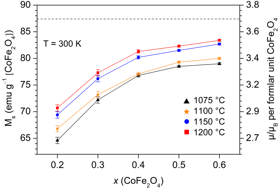
Fig. S3: Saturation magnetization ( M_s ) depending on the \text{CoFe}_2\text{O}_4 fraction ( x ) in (\text{Sr}_{0.5}\text{Ba}_{0.5}\text{Nb}_2\text{O}_6)_{1-x}-(\text{CoFe}_2\text{O}_4)_x composite ceramics sintered at the indicated temperatures for 1 h. M_s values for the composite samples were calculated by extrapolating of the magnetization at high field to H = 0 [2] and are given with respect to the nominal \text{CoFe}_2\text{O}_4 content. The black dotted line represents the M_s value of pure bulk \text{CoFe}_2\text{O}_4 , synthesized under the same conditions.
