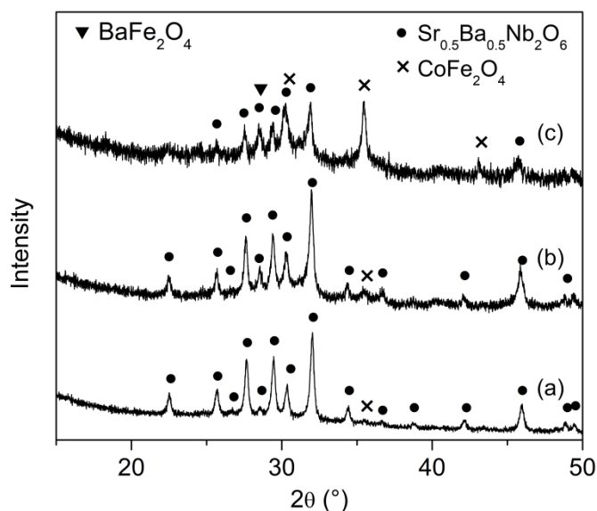
Fig. 1: Room-temperature XRD patterns of selected (\text{Sr}_{0.5}\text{Ba}_{0.5}\text{Nb}_2\text{O}_6)_{1-x}\text{--}(\text{CoFe}_2\text{O}_4)_x composite powders after calcining at 700^\circ\text{C} for 2 h (heating rate 10\text{ K min}^{-1} ): a) x = 0.2 , b) x = 0.4 , c) x = 0.6 .
