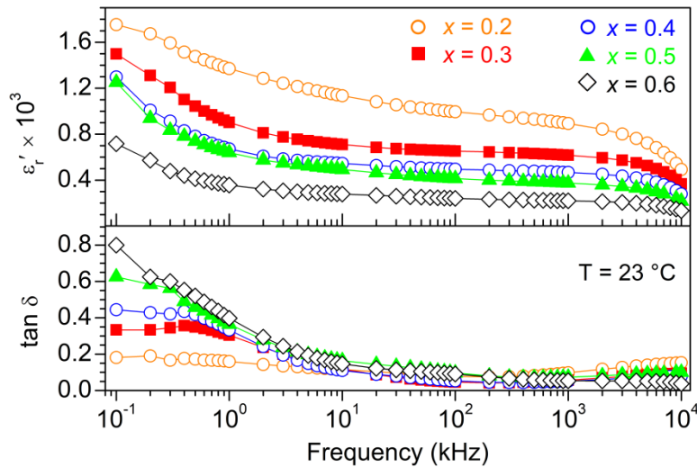
Fig. 9: Frequency dependence of the real part of the permittivity ( \epsilon_r' ) and \tan \delta at room temperature of (Sr_{0.5}Ba_{0.5}Nb_2O_6)_{1-x}-(CoFe_2O_4)_x ceramic bodies sintered at 1100\text{ }^\circ\text{C} .
