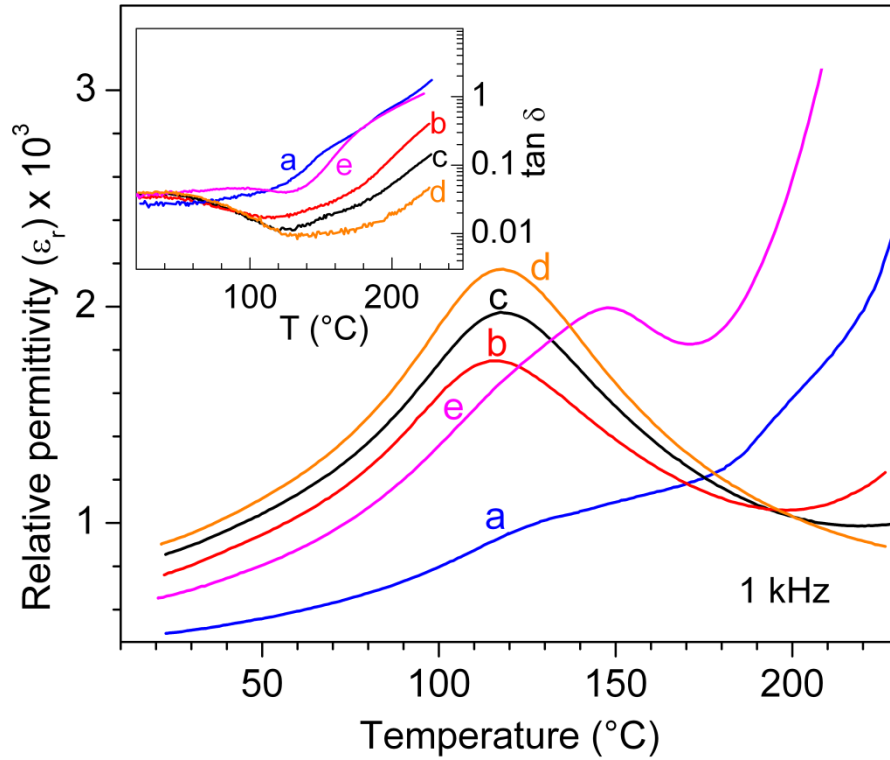
Fig. S2: Dielectric behavior of \text{Sr}_{0.5}\text{Ba}_{0.5}\text{Nb}_2\text{O}_6 of ceramic bodies sintered at different temperatures for 10 h. a) 1200 °C, b) 1250 °C, c) 1300 °C, d) 1325 °C, e) 1350 °C (from ref. [1])
