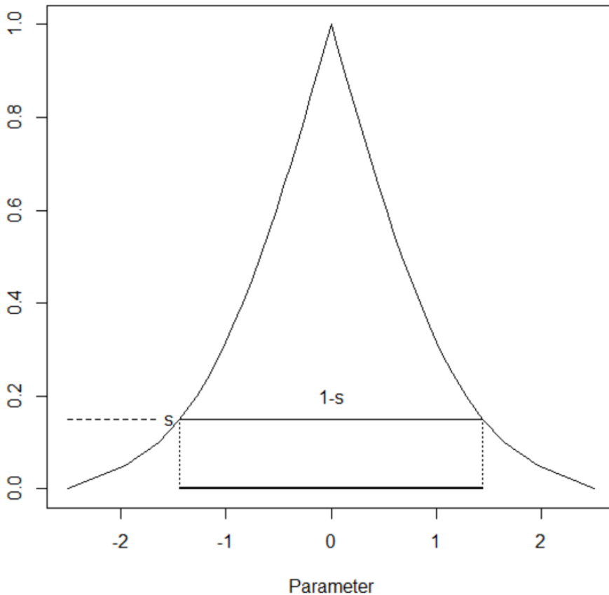
Fig. 1. For each s the line between the two branches of the curve determines a 1-s confidence interval (the thick line).
