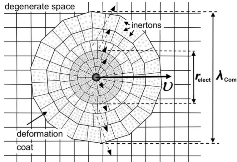
Figure 1. Moving particle in the tessellattice (degenerate space). The deformation coat shields the particle from the degenerate tessellattice. r_{\text{elect}} depicts the size of the electrically polarised sub-coat (in the case of the electron, it is Thomson's classical electron radius; \lambda_{\text{Com}} illustrates the deformation sub-coat induced by the particle mass (it is definitely the Compton wavelength of the particle). The moving particle manifests itself as a wave, covering the environment with spatial excitations – inertons.
