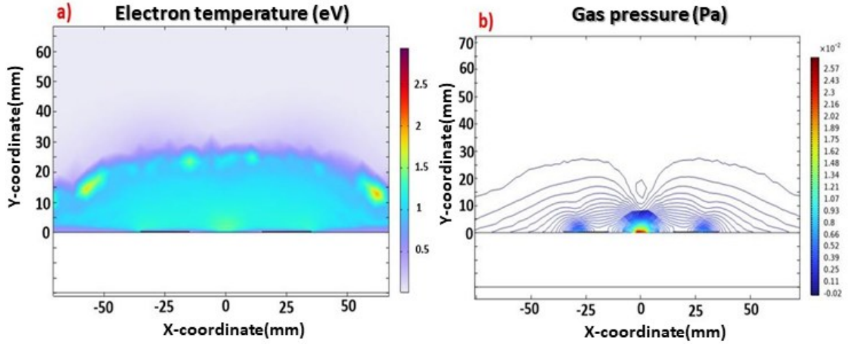
Figure 16. Simulated two-dimensional changes in a) electron temperature (eV) and b) gas pressure (Pa) at the end of two cycles.
