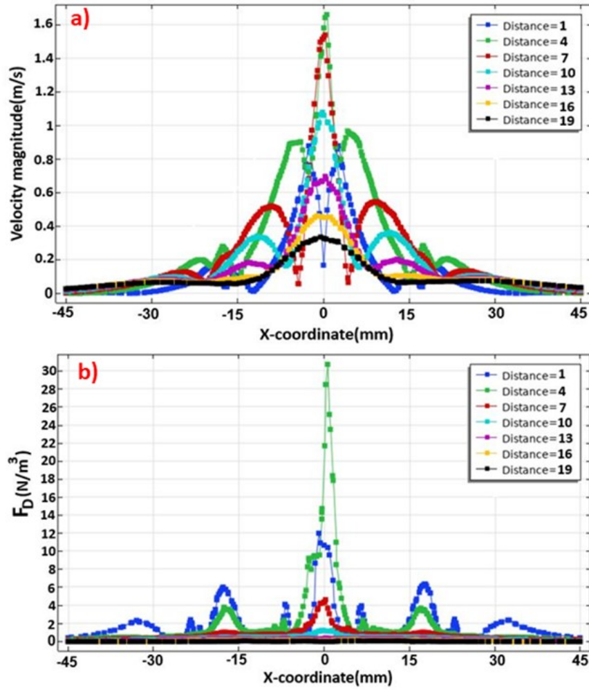
Figure 15. Simulations of a) fluid velocity, b) volumetric force under conditions of separated lines, y-axis from 1 to 20 mm, and x-axis from -45 to 45 mm.
