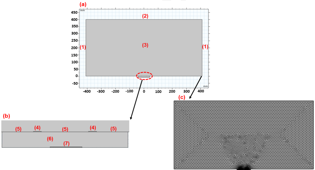
Figure 2. (a) Overall computational region, (b) close-up view of the plasma formation region, (c) meshing structure
