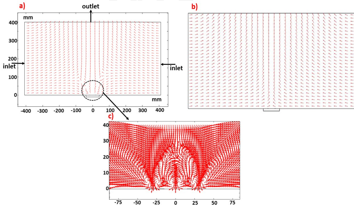
Figure 13. How the gas-fluid field lines are distributed in the conditions of (a) plasma on, (b) plasma off, (c) on plasma from a close-up view of the plasma region.
