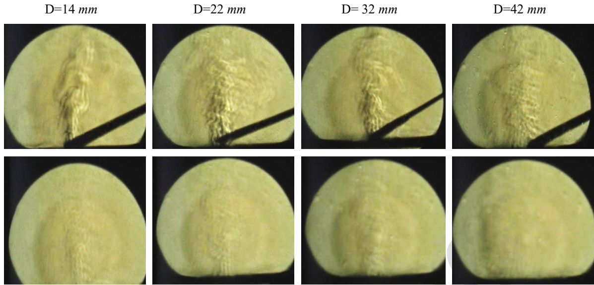
Figure 112. Schlieren image taken from SDBD with different diameters and thickness of 0.06 mm at a peak-to-peak voltage of 16 kV and a frequency of 18.9 kHz with and without the presence of scented incense (the dimensions of the images are 6 * 8 cm).
