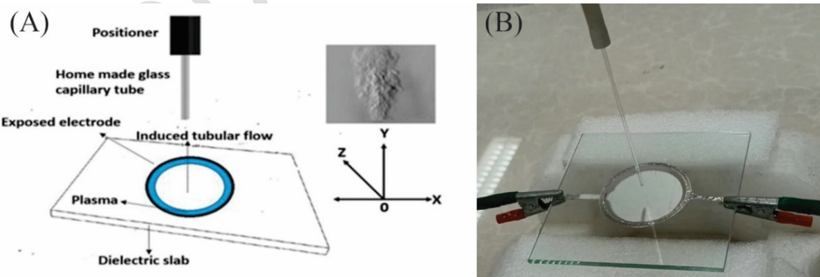
Figure 3. (A) Schematic and, (B) real picture of measuring electric wind velocity perpendicular to the surface electrode plane.
