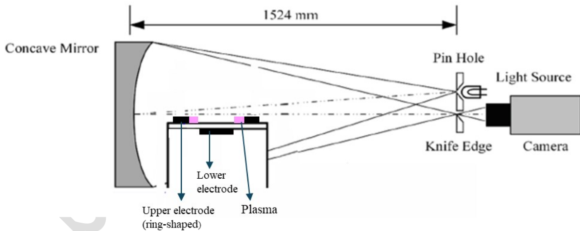
Figure 5. Cross-section schematic of Schlieren imaging.
