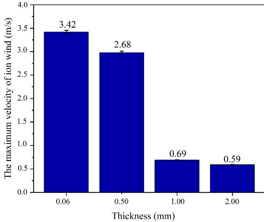
Figure 10. Graph of the maximum velocity of ion wind obtained in actuators with a fixed electrode diameter of 32 mm and different thicknesses at a fixed height of 5 mm.
