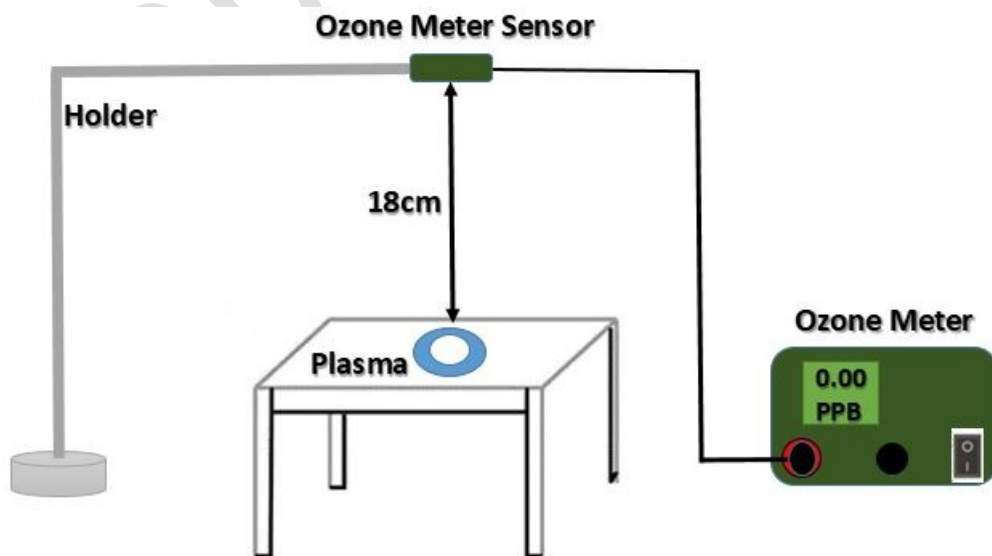
Figure 4. Schematic of the ozone meter and how its sensor is placed above the actuator.
