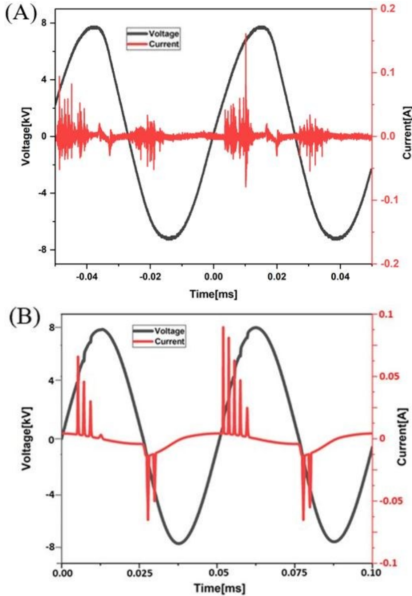
Figure 12. The voltage-current characteristic curve, (A) experimental, (B) simulation, for the electrode with a diameter of 32 mm.
