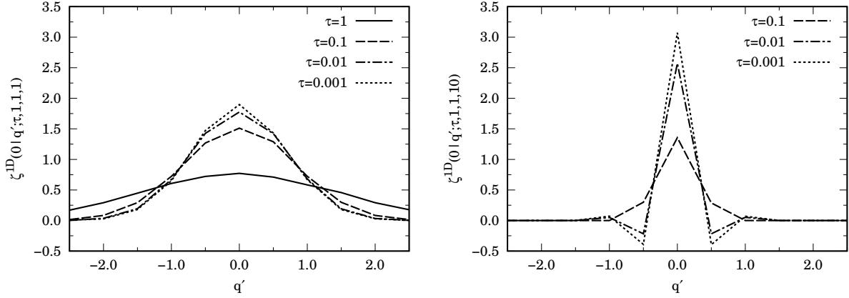
FIG. 3. We show the one dimensional \zeta^{1D}(q|q';\tau,m,\xi) calculated with a Monte Carlo scheme using 10^7 (with the related statistical error) sampling points and choosing smaller and smaller timestep \tau . All the four integrations over the ghost variables (q_a, p_a) and (q_b, p_b) were chosen in the interval [-l, l] , l = 10 (with the related finite size error). On the left m_{h.o.} = 1 on the right m_{h.o.} = 10 . Note that the slight negative values for the high m_{h.o.} and small \tau case are numerical artifacts due to the finite size, l < \infty , error.
