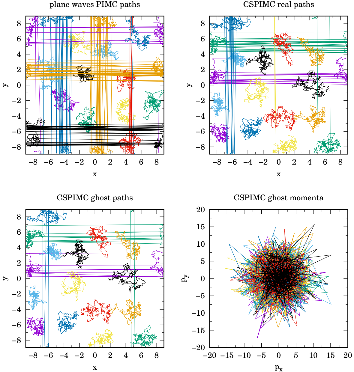
FIG. 2. We show a snapshot at equilibrium for the paths in the plane wave PIMC and the real paths, ghost paths, and ghost momenta for the CSPIMC for N = 16 {}^4\text{He} atoms ( m = 0.08306 \approx 1/12 \text{ \AA}^{-2}\text{K}^{-1} ) in two dimensions interacting with a Lennard-Jones pair potential with parameters [35] \sigma = 2.556 \text{ \AA} , \varepsilon = 10.22 \text{ K} and a cutoff distance r_{\text{cut}} = 2.5 \text{ \AA} , at a density N/L^2 = 0.05 \text{ \AA}^{-2} and a temperature T = 1.0 \text{ K} with M = 250 , 2\xi = 40 , \varphi = 24/25 in Boltzmann statistics. Different colors refer to different real or ghost atoms.
