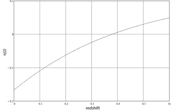
Figure 2: Graph of the function \eta(z) = \mu_2(z, 73, 0.34) - \mu_1(z, 67.6, 0.9) with \langle |\eta(z)| \rangle = 0.055 .
