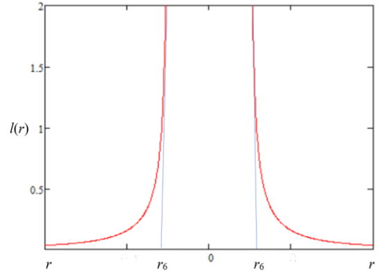
Fig. 7: Graphic functions (223) l_r^{(+)} = \frac{\Delta r}{r}
