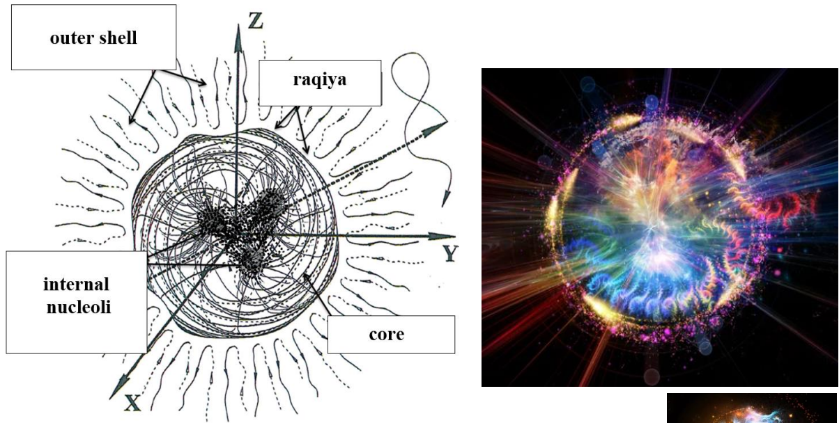
Fig. 11: Illustration of a concave on average spherical stable vacuum formation, consisting of two colored "antiquarks" and one "quark" (specifically, a p_i^- - "proton" (250)). The inner nuclei of these vacuum formations are in constant, chaotic motion relative to each other and relative to the common center of the p_i^- - "proton's" core
