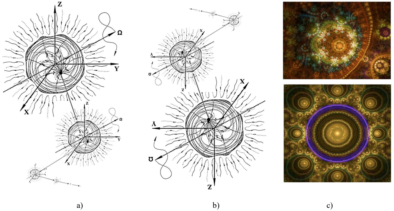
Fig. 3: a) A hierarchical 10-level chain of different-scale "corpuscle" cores (i.e., convex spherical vacuum formations) nested inside each other like Russian dolls; b) An inverted hierarchical 10-level chain of different-scale "anticorpuscle" cores (i.e., concave spherical vacuum formations) nested inside each other like Russian dolls; c) Fractal illustrations of "cores in Cores"
