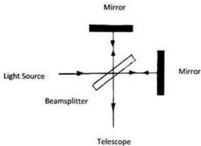
Figure 4: Michelson-Morley Apparatus
