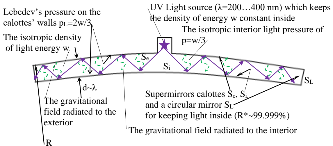
Fig.2-The scheme of a high-frequency gravitational waves generator
