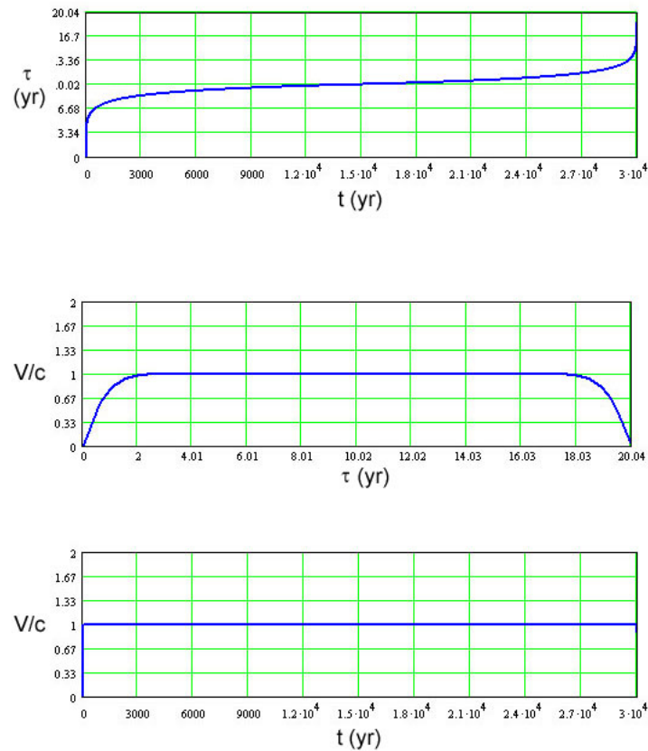
Figure-3, Proper time verses time, velocity verses proper time and velocity verses time
