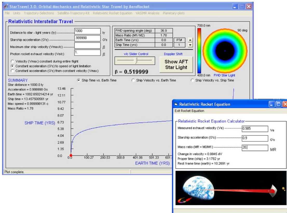
Figure-1, Time Dilation and Doppler light shift analysis 7 showing forward (FWD) star colors.
