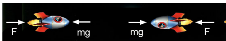
Figure-2, Acceleration leaving Earth then deacceleration at half-way point
