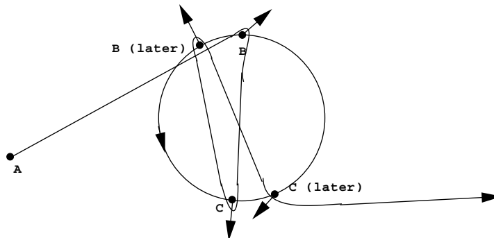
Figure 2. Detailed behavior during "type 1" interaction of asteroid with binary. Stars B and C are rotating happily in the roughly circular orbit shown. Asteroid A swings past star B then past star C, then B again (later in its orbit) and then finally C (again) and then begins the long trek along the N-gon edge toward the next binary. During the 4 hyperbolic swingbys, 4 momentum transfers from the asteroid to the star occur, roughly as shown by the vectors. The total effect of these momentum transfers has a component in opposition to the orbital velocity of the stars. Note: some distances have been exaggerated for clarity. In fact, the angular separation between B and B(later) or between C and C(later), is O(\mu) (that is, small), and the separation between the asteroid and any star at the point of closest approach, is extremely small, so that the trajectory should in fact look much more like a chain of 5 line segments, than it does.
