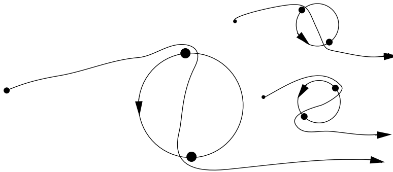
Figure 3. Detailed behavior of "type 2" interaction of asteroid with binary. this simple trajectory was the one originally proposed by Gerver and it has the same sort of energy transfer properties as our alternate proposal in figure 2, in the limit when \mu is small. Incidentally, in figures 2 and 3, the range of initial phase angles is quite flexible (there is a range of size nearly \pi ), as is shown in the two smaller alternative versions of the present figure that are off to the right. This flexibility is essential to keep control of the eccentricity of the (slightly elliptical) orbit.
