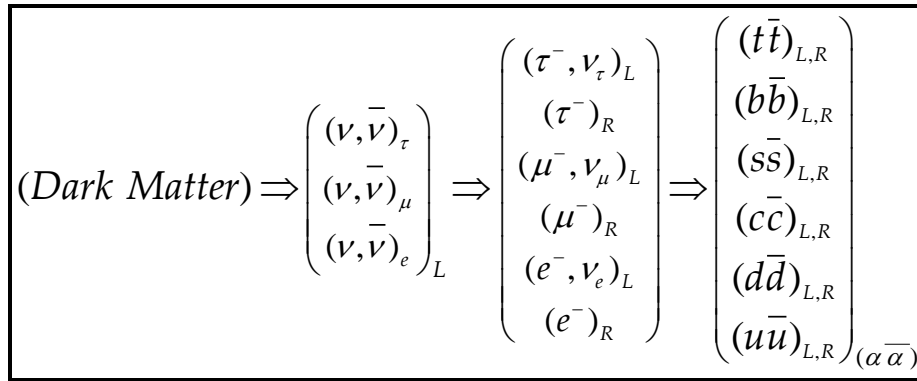
Fig. 1 Bifurcations of Dark Matter into neutrinos and charged fermions [5]
