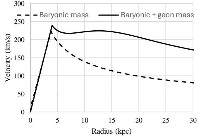
Figure 3. Calculated velocity profiles for the Milky Way (simplistic model), showing the Newtonian decay and the relatively flat profiles obtained by the additional force of the geon.
