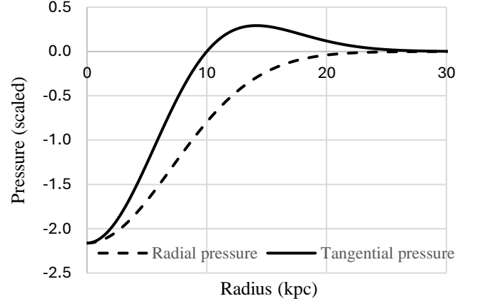
Figure 2. Radial and tangential pressure profiles of the geon. The units are scaled; the pressures (in Pa) are obtained by multiplying the scaled values by 10^{-38} .
