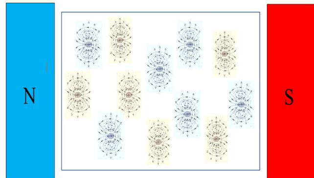
Fig. 13. Toroidal vacuum vortices (i.e. cluster magnetic fields) are induced in distilled water located between the poles of a magnet.
