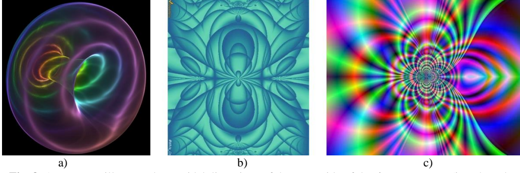
Fig. 8. Attempts to illustrate the toroidal distortions of the outer side of the \lambda_{-12,-15} -vacuum (i.e., the subcont) in the vicinity of the center of the electron "neutrino" in the final state
