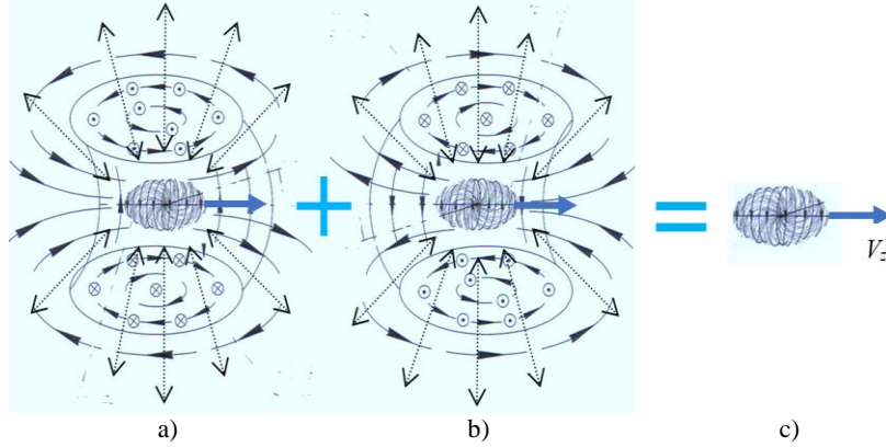
Fig. 1. (Repetition of Figure 7 in [8]). In the outer shell (more precisely in the vicinity of the core) of the “electron” moving with a constant velocity V_z on average, two counter toroidal-helical subcont vortices and two counter (inflowing and outflowing) subcont laminar currents are induced, which compensate each other's manifestations. Therefore, only the moving core of the “electron” can be observed
