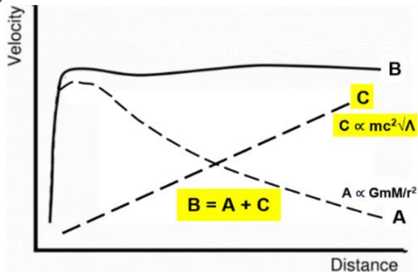
Fig. 9. Galaxy rotation curve (B) as a result of two forces: the contribution of the Newtonian force (A) and the contribution of the cosmological force (C).
