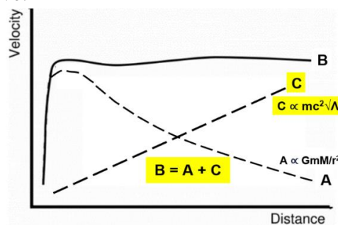
Fig. 8. Galaxy rotation curve (B) as a result of two forces: the contribution of the Newtonian force (A) and the contribution of the cosmological force (C).
