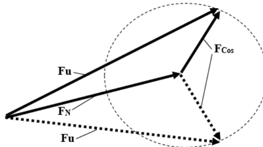
Fig. 6. The force of universal gravitation F_U as a vector sum of two forces: F_N and F_{Cos} .
