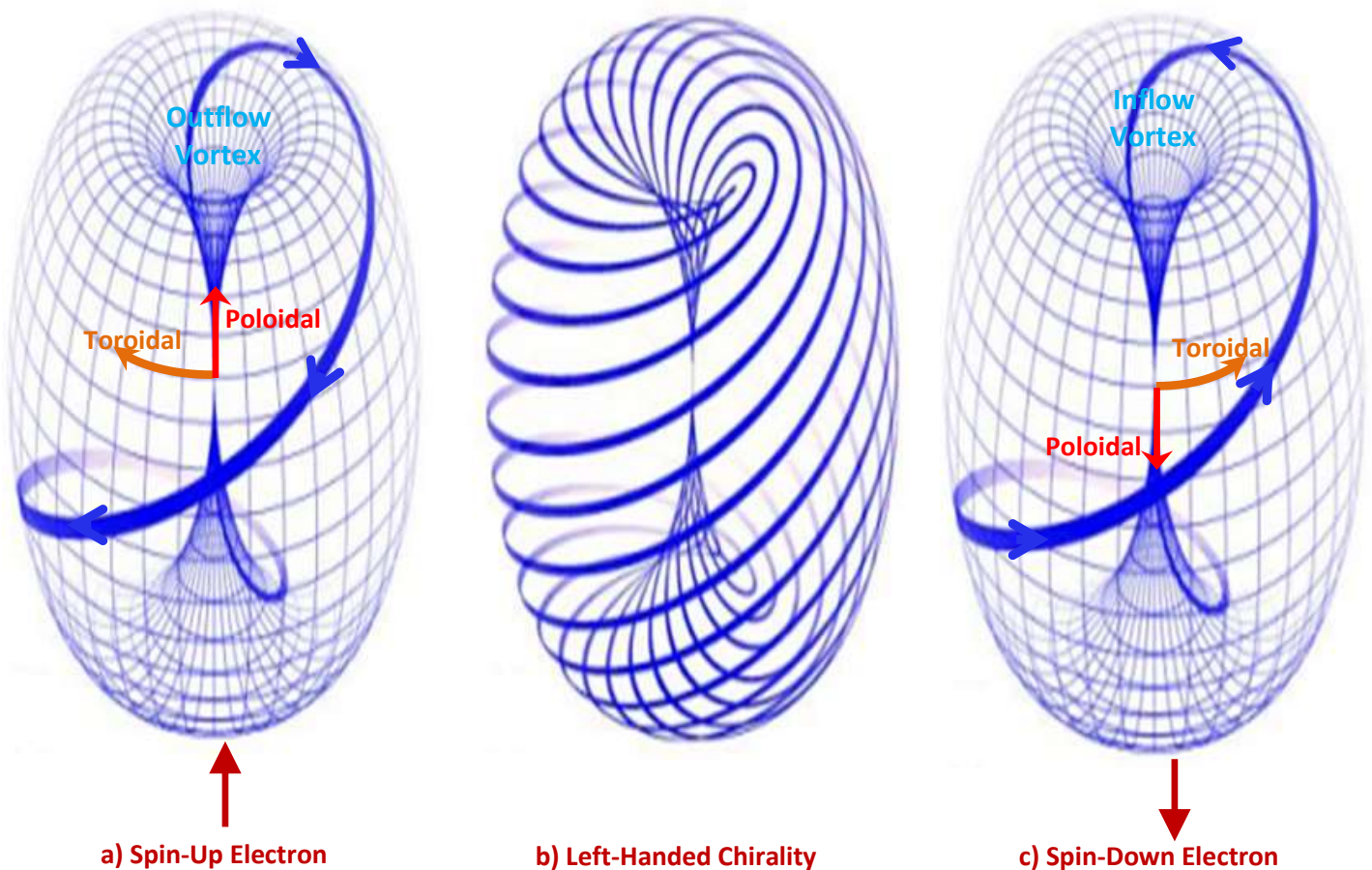
Figure 5: Chirality and Spin-Up/Spin-Down Electrons
