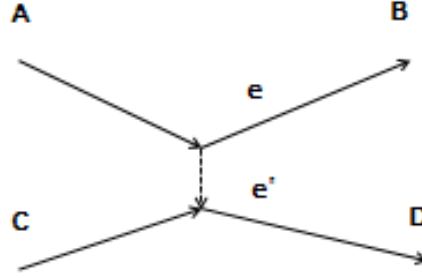
FIGURE 4. scattering e-e
