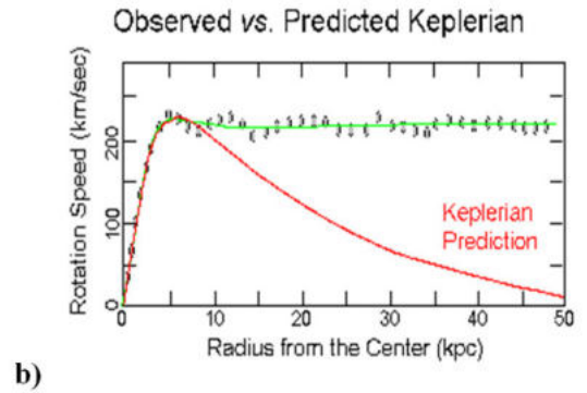
Figure: Dependencies of velocity of rotation of astronomical objects on the distance to gravity center: a) our Milky Way galaxy (Bennett et al., 2012; Rieke, 2016), b) comparing to prognosed Keplerian velocities (Thompson, 2011)
