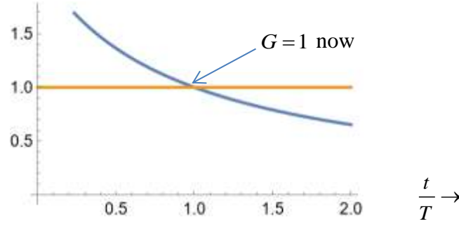
Figure 8.2.7 A plot of the gravitation parameter G starting at G = 2.14 in Planck units.
