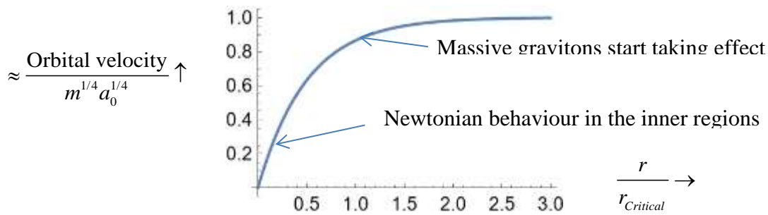
Figure 8.1.1 Plot of a very hypothetical orbital velocity radial profile assuming the peak radial mass densities, where the massive gravitons originate, are somewhere greater than one Milgrom critical radius. This behaviour has many parallels to MOND predictions.
