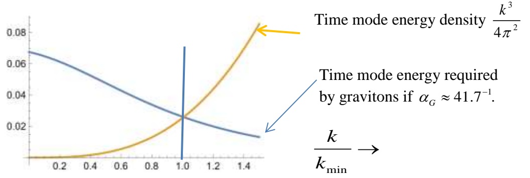
Figure 8.2.8 A plot of the time mode energy density \frac{k^3}{4\pi^2} and that required by gravitons if \alpha_G \approx 41.7^{-1} . For all k > k_{\min} the time mode energy required by gravitons can come from the normal supply. But for all k < k_{\min} , they must come from the Hubble flow expanding space supply as in the section 5.3.1 and Eqs. (5.3.16) and (5.3.17). Because both G & \alpha_G vary with cosmic time this plot will also look different in other eras.
