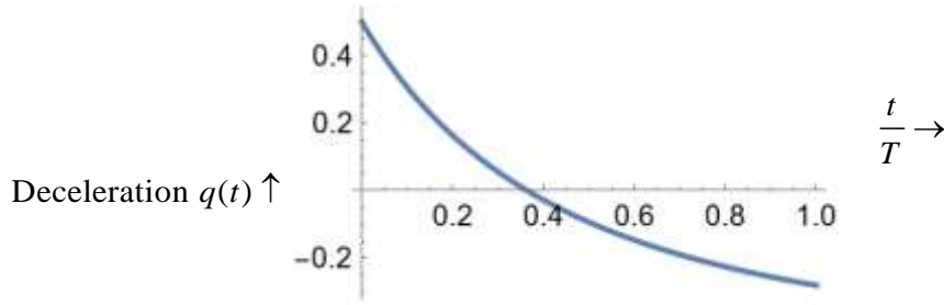
Figure 8.2.2 Deceleration as a function of cosmic time with d = 1 in Eq.,(8.2.24)
