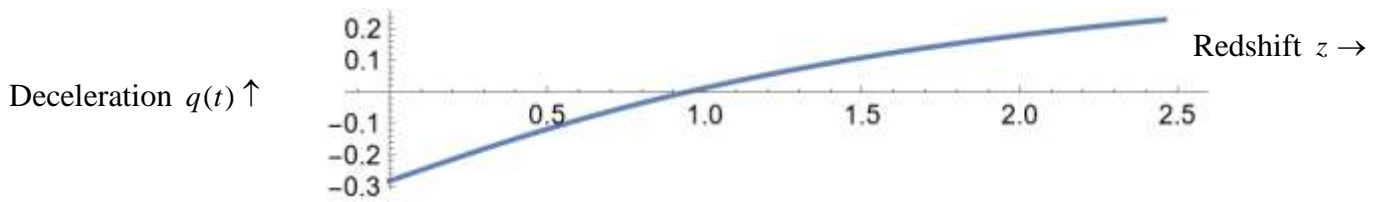
Figure 8.2.5 A plot of deceleration versus redshift, with z_t \approx 0.9 at transition.
