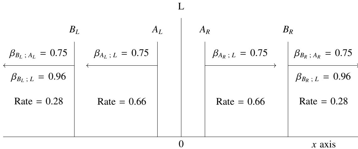
Figure 1: The scenario as seen from reference frame L , the lab (“stationary”) frame. The rates shown are fractional clock rates as compared to the rates of clocks in lab frame L . Note the symmetry about the lab frame y axis.
