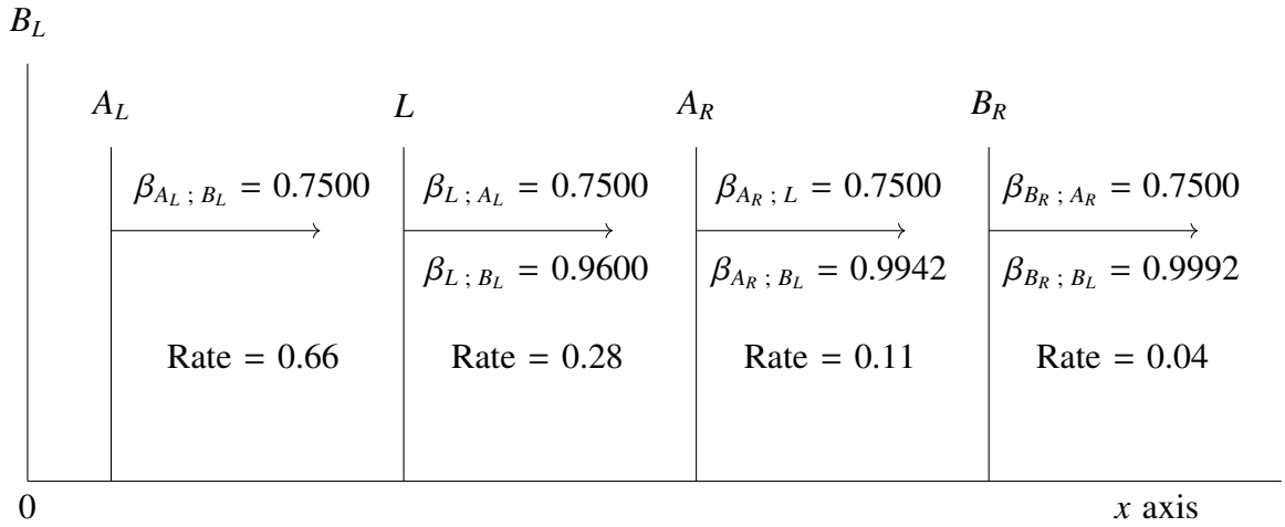
Figure 2: The scenario as seen from reference frame B_L . The rates shown are fractional clock rates as compared to the rates of clocks in reference frame B_L . Note the absence of the symmetry shown in the previous figure.
