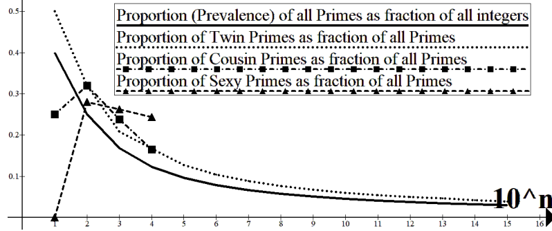
9 Proportion (Prevalence) of Twin primes, Cousin primes [as partial calculations] and Sexy Primes [as partial calculations] with Proportion (Prevalence) of all Primes included. These Proportions (Prevalences) are essentially self-similar fractal objects . The n = 1, 2, 3, 4, 5, 6, 7, 8, \dots in 10^n that is denoted with horizontal x-axis \implies the scale of this axis is non-linearly depicted using increasing powers of 10.
