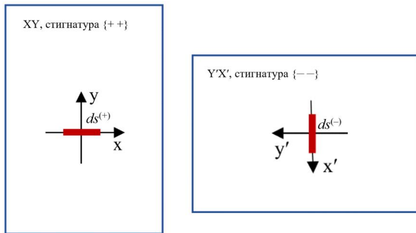
Fig. 11: Two sides of the space with completely opposite stignatures \{++\} and \{--\}
