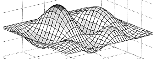
Fig. 14: 2D-illustration of a convex-concave two-sided surface with signatures \{++\} and \{-+\} . This curved surface is such that it is, on average, flat. At the same time, the deformation that looks like a convexity from the outside, from the inside it looks like a concavity. At the same time, it should be taken into account that if the signatures of the sides of such a two-sided surface are completely opposite \{++\} and \{--\} , then the deformations on its two sides are not only mutually opposite, but also mutually perpendicular (see §5.2)
