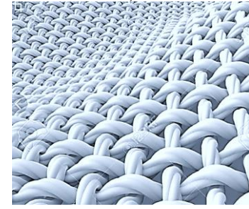
Fig. 12: Woven threads of the fabric
