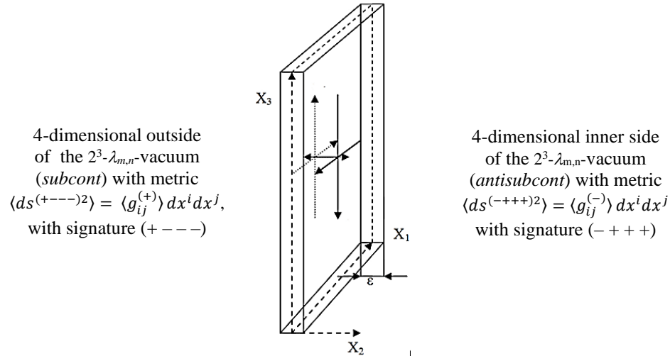
Fig. 7: Simplified illustration of a two-sided section of the 2^3\text{-}\lambda_{m,n} -vacuum, the outer side of which ( subcont ) is described by the averaged metric \langle ds^{(+---)^2} \rangle (30) with the signature (+---) , and its inner side ( antisubcont ) is described by the metric \langle ds^{(-+++)^2} \rangle (33) with the opposite signature (-+++) , as \epsilon \rightarrow 0
