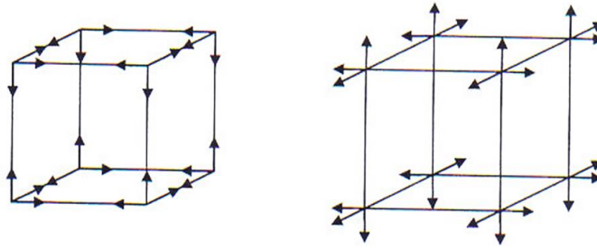
Fig. 9: A cube isolated in the thickness of a sheet of paper (or in some other continuous medium, including vacuum)
