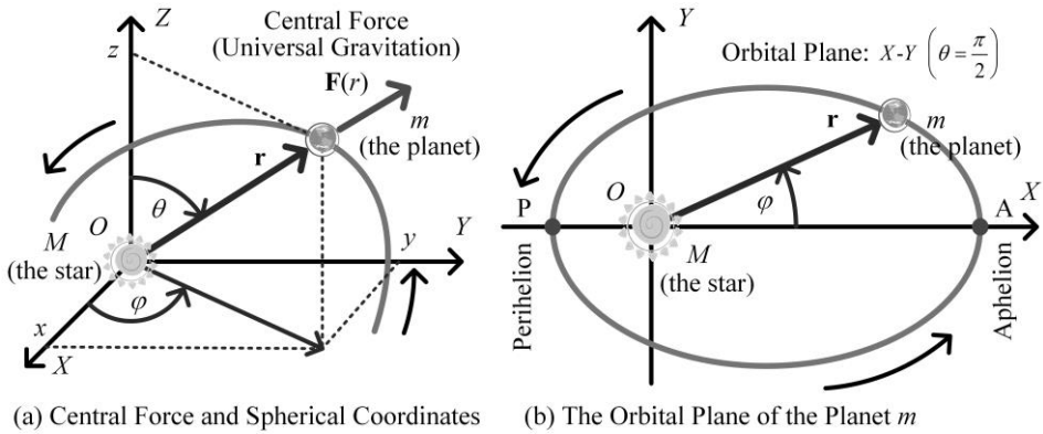
Figure 16.2 The Formalized Coordinates of Celestial Two-Body Problem. (a) Central force and spherical coordinates: The two-body system (M,m) of celestial bodies is idealized as an isolated system in the space of spherical-coordinate O(r, \theta, \varphi) , where the large mass celestial-body M (the sun or a star) is located at the coordinate origin of O , and the small mass celestial-body m (a planet or comet or satellite or even photon) moves in the gravitational field of M ; universal gravitation is a sort of central force that always points towards the large mass celestial-body M (at the coordinate origin O ). (b) The orbital plane of the small celestial-body m : According to the property of central force, the motion of the particle m is limited to a fixed plane.
