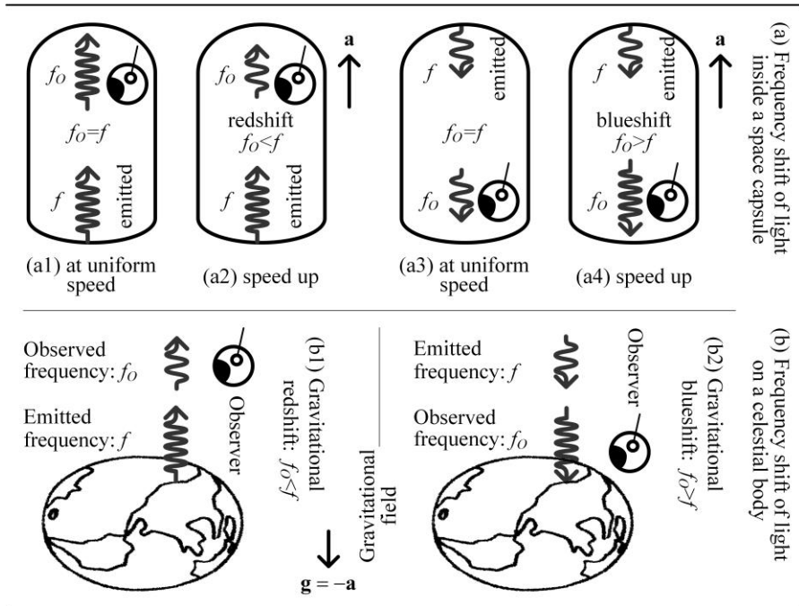
Figure 18.1 Equivalence Principle and Gravitational Redshift. (a) The frequency shift of light inside a spacecraft: As the spacecraft travels at uniform speed, the light source stationary in the spacecraft emits light with the frequency f which is constant relative to the astronauts inside the spacecraft ( f_o=f in (a1) and (a3)); as the spacecraft accelerates, the astronaut at the front finds that the frequency f of the light emitted by the light source at the rear presents decay or redshifts ( f_o<f in (a2)), while the astronaut at the rear finds that the frequency f of the light emitted by the light source at the front presents growth or blueshift ( f_o>f in (a4)). (b) Frequency shift of light on a celestial body: According to Einstein’s equivalence principle, the astronauts inside the spacecraft could not distinguish whether the spacecraft is in an accelerated state or in a gravitational field, and therefore, for a massive celestial body (a gravitational field \mathbf{g}=-\mathbf{a} in (b)), the observer would find that the frequency f of the light flying from the celestial body towards the inertial space must present decay or redshift ( f_o<f in (b1)), while the observer would find that the frequency f of the light flying from the inertial space towards the celestial body must present growth or blueshift ( f_o>f in (b2)).
