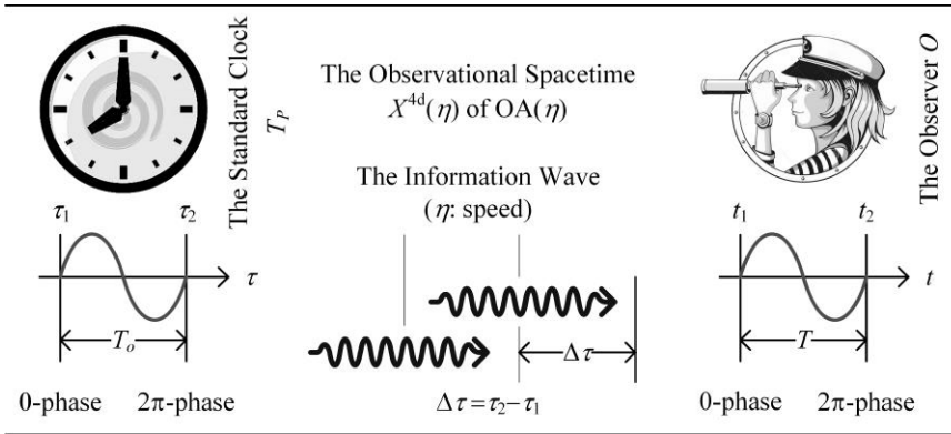
Figure 13.1 The Observer O and the Observed Time t : The observer O observes the standard clock T_P ; the time dt observed by O depends on the general observation agent OA(\eta) that O is armed with. The general observation agent OA(\eta) has the observational locality ( \eta<\infty ), and therefore, the observed time dt is not the objectively real time d\tau . However, in the Cartesian spacetime X^{4d}_\infty , the observation agent is the idealized agent OA_\infty ( \eta\rightarrow\infty ), and has no observation locality, thus dt=d\tau .
