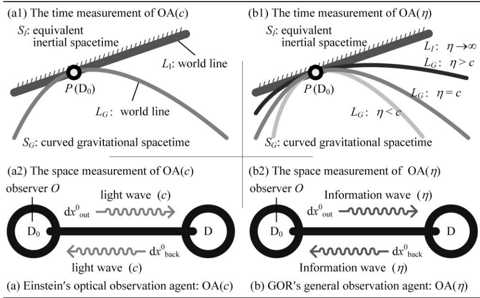
Figure. 12.1 The Measurement of Observational Spacetimes. (a) The observational spacetime of Einstein general relativity: it employs the optical observation agent OA(c) to measure time and space; the speed c of light is limited ( c < \infty ), and therefore, OA(c) has the observational locality and the gravitational spacetime looks a little curved. (b) The observational spacetime of GOR: it employs the general observation agent OA(\eta) to measure time and space, the slower the information-wave speed \eta , the more significant the observational locality of OA(\eta) , the more curved the gravitational spacetime appears; under the idealized observation agent OA_\infty , as \eta \rightarrow \infty , without observational locality, the gravitational spacetime would revert to flat.
