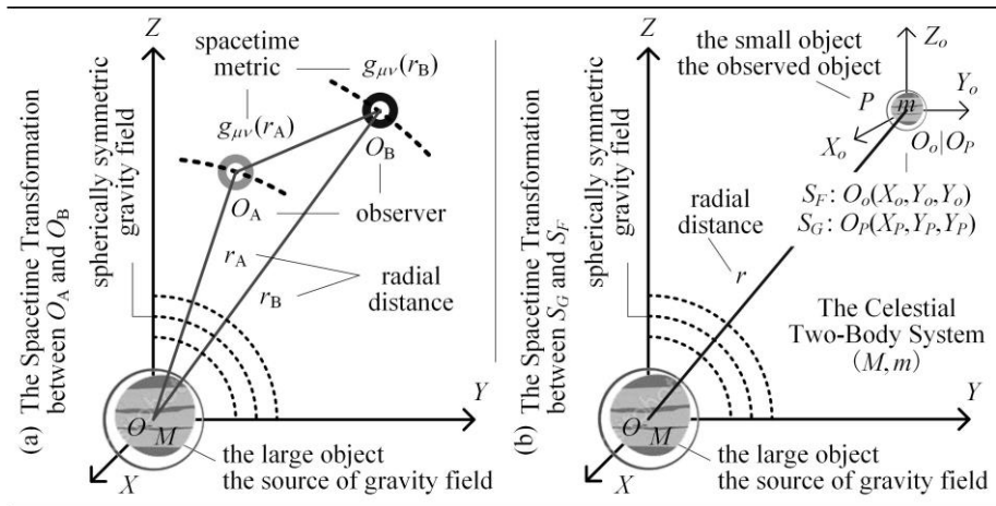
Figure 10.1 The Scene of GOR Gravitational Spacetime: the Celestial Two-Body System (M,m) . (a) The Spacetime Transformation between the Observers O_A and O_B : the points A and B in the gravitational spacetime S_G have different spacetime metrics g_{\mu\nu}(r_A) and g_{\mu\nu}(r_B) , and therefore, the observational spacetimes of O_A and O_B are different, which need to be transformed. (b) The Spacetime Transformation between the gravitational spacetimes S_G and the Free Spacetime S_F : according to Def. 1.2, the physical quantities of the observed object P at rest in free spacetime S_F are the objective and real physical quantities of P , but the physical quantities of P observed by observers in the gravitational spacetime S_G are different from the objective and real physical quantities of P , which need to be transformed.
