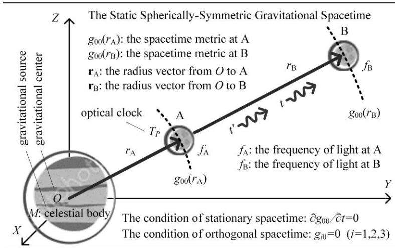
Figure 18.2 The Gravitational Redshift of Light in A Static Spherically-Symmetric Gravitational Spacetime: The celestial body M is the gravitational source and the center of the spherically-symmetric gravitational spacetime. The light source or optical clock T_P at the point A stationary in the gravitational spacetime of M emits the light signal with the frequency f_A to the point B. The observer at the point B receives the light signal with the frequency f_B . According to Einstein's equivalence principle and Einstein's theory of general relativity: f_B < f_A , which means that the frequency of the light signal decays in gravitational spacetime, showing the phenomenon of gravitational shift.
