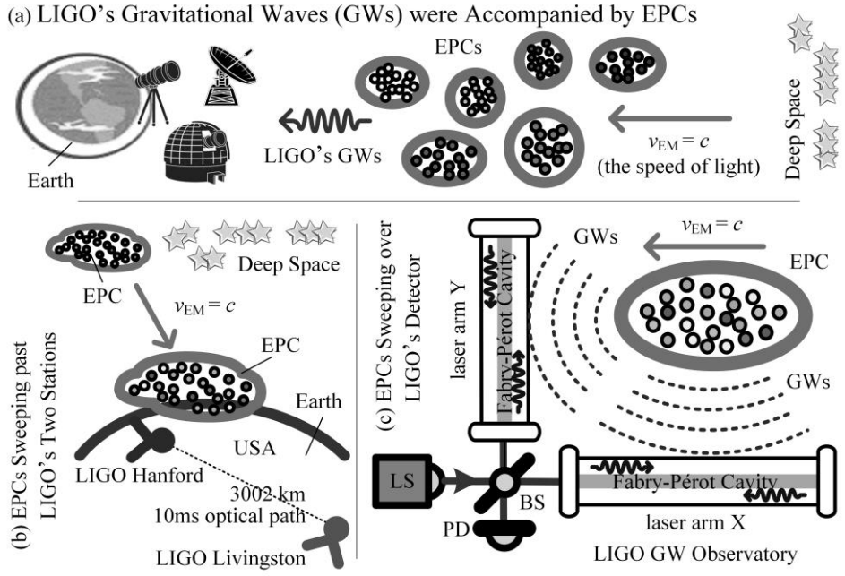
Figure 19.4 Why were LIGO's Gravitational Waves Always Accompanied by EPCs? (a) LIGO's Gravitational Waves were Accompanied by Electromagnetic Matter: Whenever LIGO detected a gravitational-radiation signal, it would always be found that there were some electromagnetic-particle clumps (EPCs) before and after it, which are known as electromagnetic counterparts, such as gamma-ray bursts and X-rays; naturally, of course, EPCs move at the speed of light. (b) The Gravitational Fields of EPCs Sweeping at the Speed of Light past the LIGO Livingston and the LIGO Hanford: As matter systems, EPCs have the gravitational fields of their own moving together with EPCs; it is not that LIGO's gravitational-radiation signals or gravitational waves moved at the speed of light, but that EPCs moved at the speed of light. (c) The Gravitational Fields of EPCs Sweeping over the LIGO Detector: If an EPC sweeps the LIGO detector at close quarters and its gravitational field asymmetrically invaded and disturbs the spacetime around the laser arms X and Y of LIGO detector, the EPC may trigger the LIGO detector; what LIGO detected were not the gravitational wave originated from the distant black hole in deep space, but the gravitational radiation of the EPC in a short distance.
