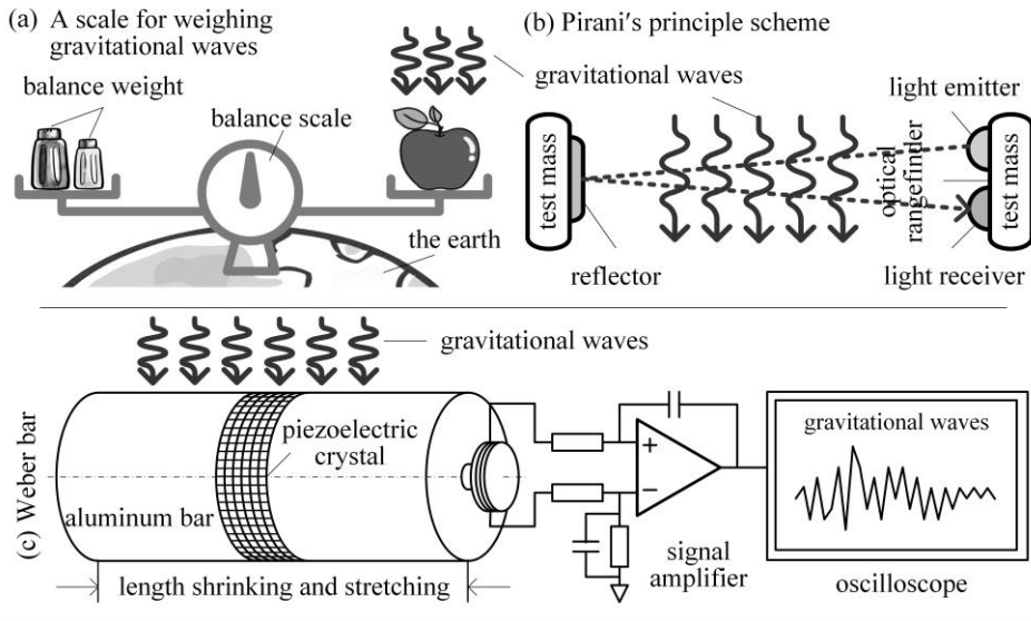
Figure 19.1 The Proof-of-Principle Scheme of Gravitational-Wave Deflection. (a) A scale for weighing gravitational waves: Perhaps, by making use of a scale, you could weigh gravitational waves just like your weighing an apple. (b) Pirani's proof-of-principle scheme: Based on Einstein's theory of general relativity, Pirani proved that gravitational waves could shrink and stretch space; therefore, as long as you have an optical rangefinder, you could measure the shrinking and stretching of Pirani length, and in this way, you could detect gravitational waves. (c) Weber bar: Inspired by Pirani's theory, Weber made the so-called Weber bar, an antenna for detecting gravitational waves; Weber believed that the shrinking or stretching of space would shrink or stretch the Weber bar, which could be detected by the piezoelectric sensors around the Weber bar and be converted into electrical signals, so that one could detect and discover gravitational waves.
