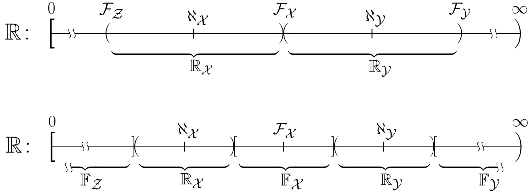
Figure 21: This figure demonstrates an open question in fractional distance analysis. Should the \mathbb{R}_\chi neighborhoods be separated by single arithmetic numbers \mathcal{F}_\chi \in \mathbb{F} (above) or should they be separated by entire neighborhoods of non-arithmetic numbers labeled \mathbb{F}_\chi (below)?
