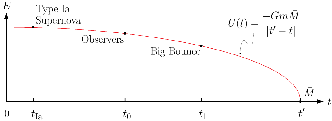
Figure 22: This figure depicts the Newtonian mechanism for MCM dark energy mostly as it appeared in [31]. t_{Ia} is the proper time of a high redshift supernova in the dark energy survey. Such supernovae live on the past light cone of an observer with proper time t_0 . The upcoming bounce lies at t_1 . t' is the temporal midpoint of the cycle of cosmology beyond the bounce and \bar{M} is a point mass representing the universe in the cycle beyond the bounce. The energy curve assumes that every slice of constant proper time in our present cycle of cosmology has the same mass m so the energy between \bar{M} and the slices of constant proper time at t_{Ia} or t_0 differs only in the timelike separation |t' - t| . Observers in an inertial frame at t_0 will see objects at t_{Ia} appear to recede under acceleration because t_0 is deeper into \bar{M} 's gravitational well.
