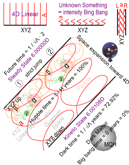
Fig. 7 Shape of quantum space
