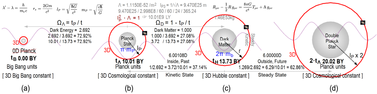
Fig. 10 Dark energy and dark matter
