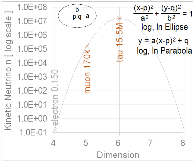
Fig. 11 Log scale of neutrinos
