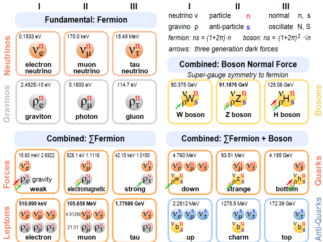
Fig. 2 New Standard Model
