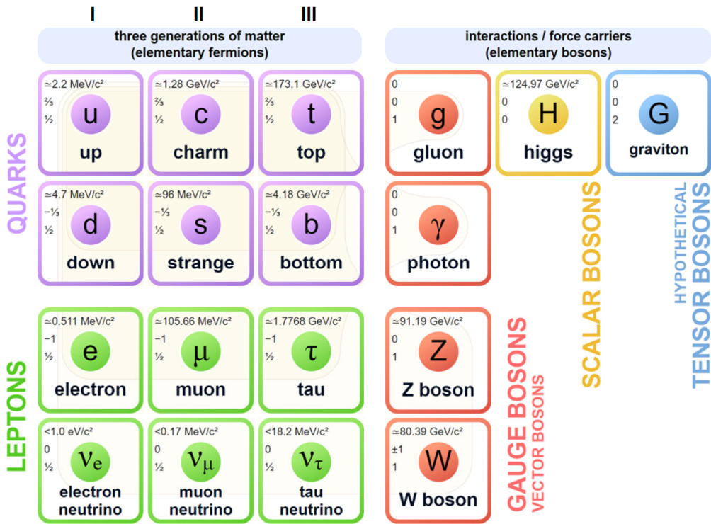
Fig. 1 Current Standard Model
