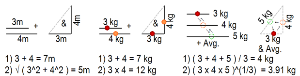
Fig. 9 Calculation of quantum particle mass
