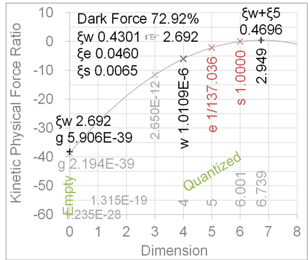
Fig. 8 Unification of four fundamental forces
