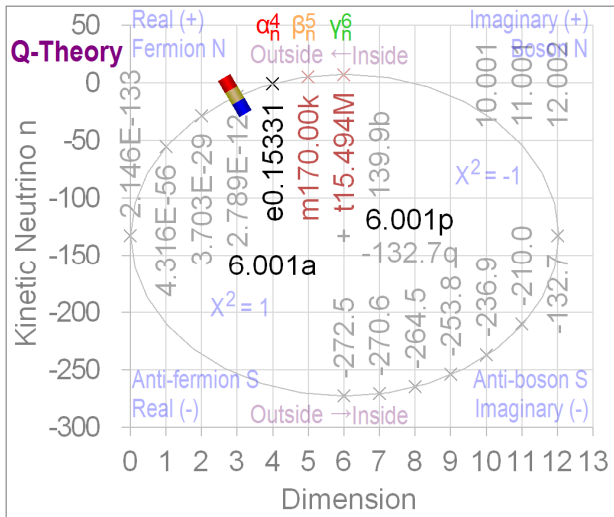
Fig. 3 Mass of normal neutrinos
