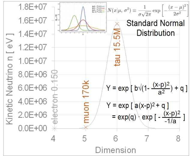
Fig. 12 Mass scale of neutrinos
