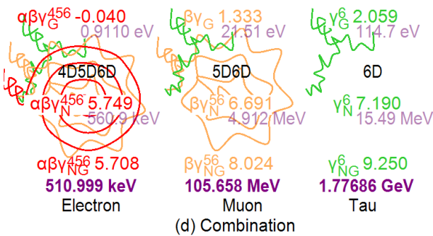
Fig. 5 Neutrinos and Leptons
