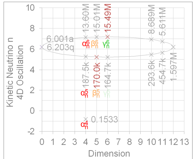
Fig. 4 Mass of oscillating neutrinos
