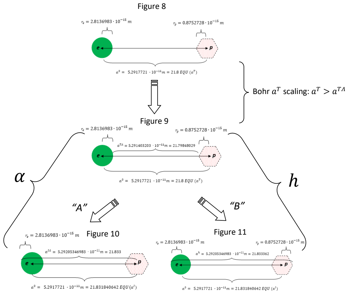
Figure 12: schematic for figures 8-11, highlighting what needs to be considered in formulating the scales for a maximum-mass (solar) event, and the two processes at play, "A" and "B".
