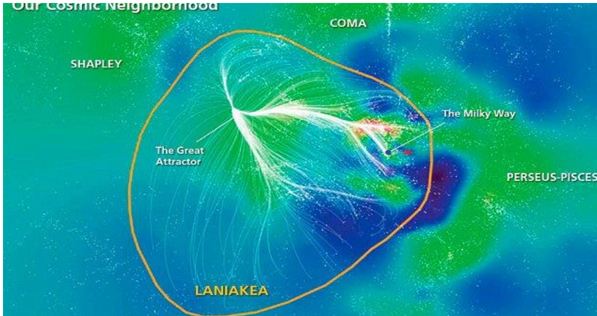
Figure 1. Laniakea Supercluster. Adapted from [46].
