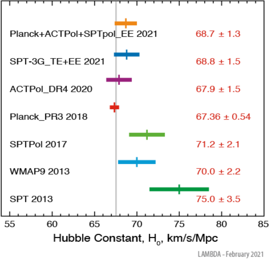
Fig. 3. Recent H_0 determinations using only Cosmic Microwave Background data. Adapted from [50],
