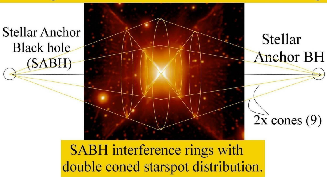
Figure 22, The Red Square Planetary nebula MWC922, equipped with double cone structure of expelled material including trailing starspots (Micro Black Holes). There are FOUR cones of interferences originated by the two Stellar Anchor black holes (SABHs). These four cones seem to interfere with the TWO cones of expelled material of the star, leading to FOUR rings of interference.
