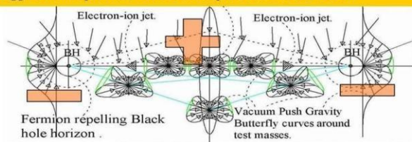
Figure 33, Secondary and Tertiary Dual BH HH systems.
