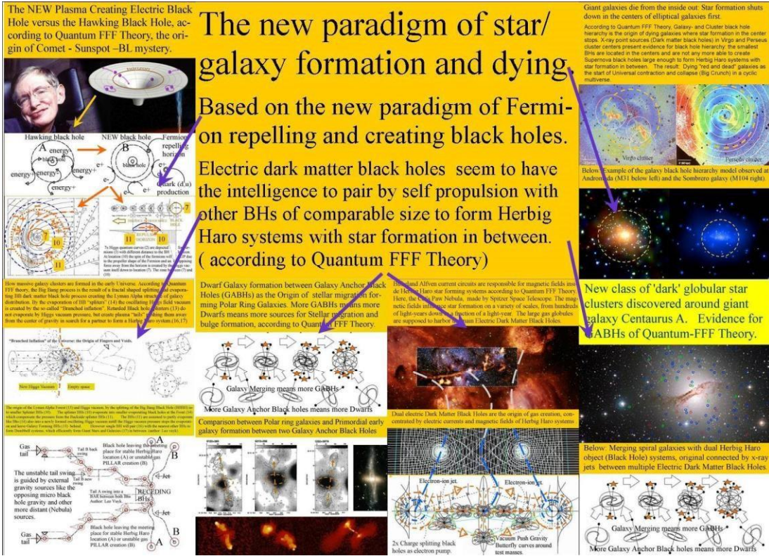
Figure 30, The new paradigm.
