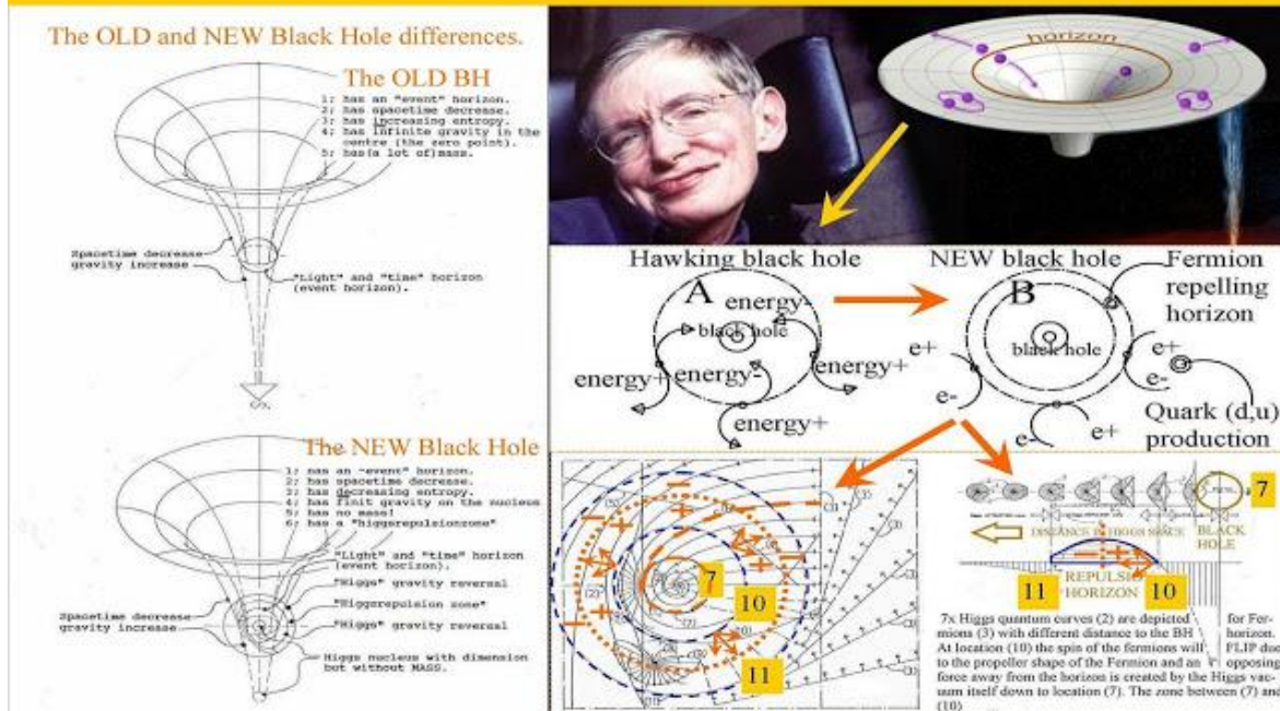
Figure 46, Negative charged Black hole at the outside, positive at the inside originated by the chiral vacuum.
