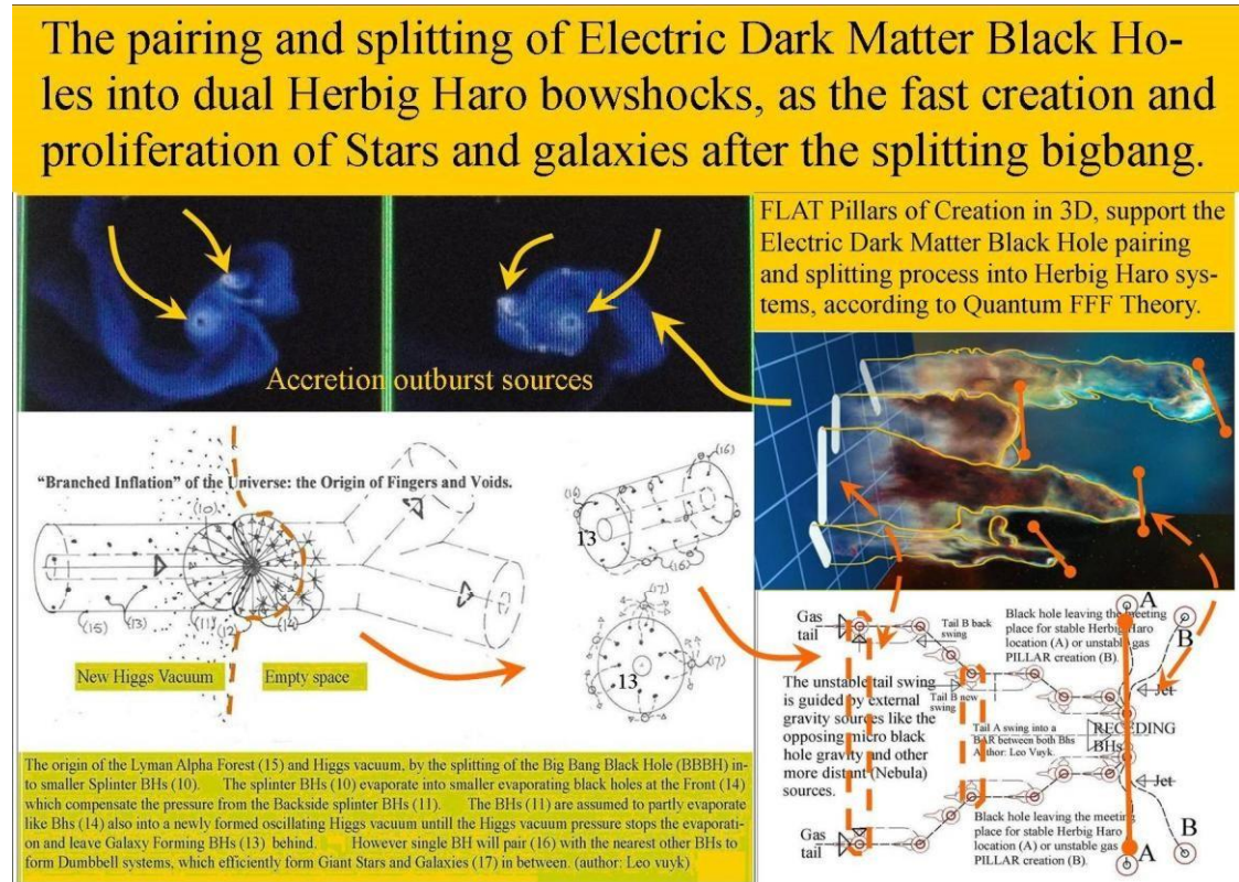
Figure 31, Examples of HH objects and dual DMBH pairing
