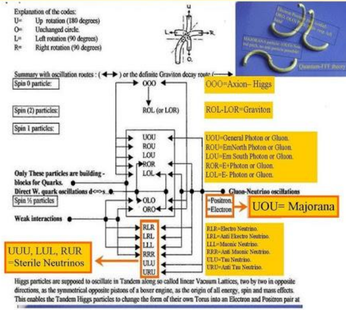
Figure 19, most rigid string particles with much dualities, ( still undiscovered) described by only three hinges and 4x possible rotations of 90 degrees. (ULRO)
