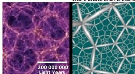
The largescale filament structure of our universe ( \rightarrow distribution of galaxies) shows similarity to a 5/3/5 honeycomb in hyperbolic 3-space. This may indicate a hyperbolic geometry of our universe.
