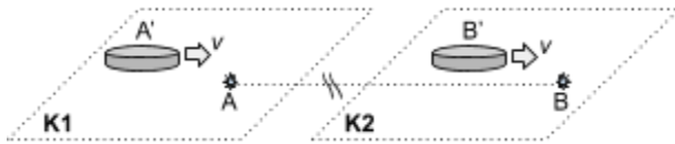
Fig 2. Setup1 to test RoS under FA. Moving frame's synchronized detectors at A' and B' pass over the vertical flash sources, A and B to record the time of the flashes in the moving frame.
