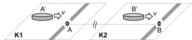
Fig 3. Setup2 to test RoS under FA. Moving detectors A' and B' are enabled by spatially limited gray metal strips engraved about A and B for a short duration.
