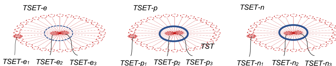
Figure 5: standard Kaon pairings (solid blue rings), and the weaker Kaon pairing of the TSET-e_2 and TSET-e_3 particles (broken blue ring).
