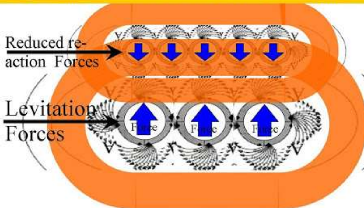
Figure 6, Anti Maxwell B=0 tubular field around a conductor s. Different diameter conductors screening small conductors to create reduced reaction less Lorentz forces.
