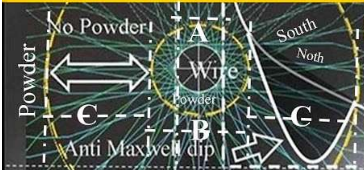
Figure 16, estimated differences between B=0 tubular boundaries around a conductor.
