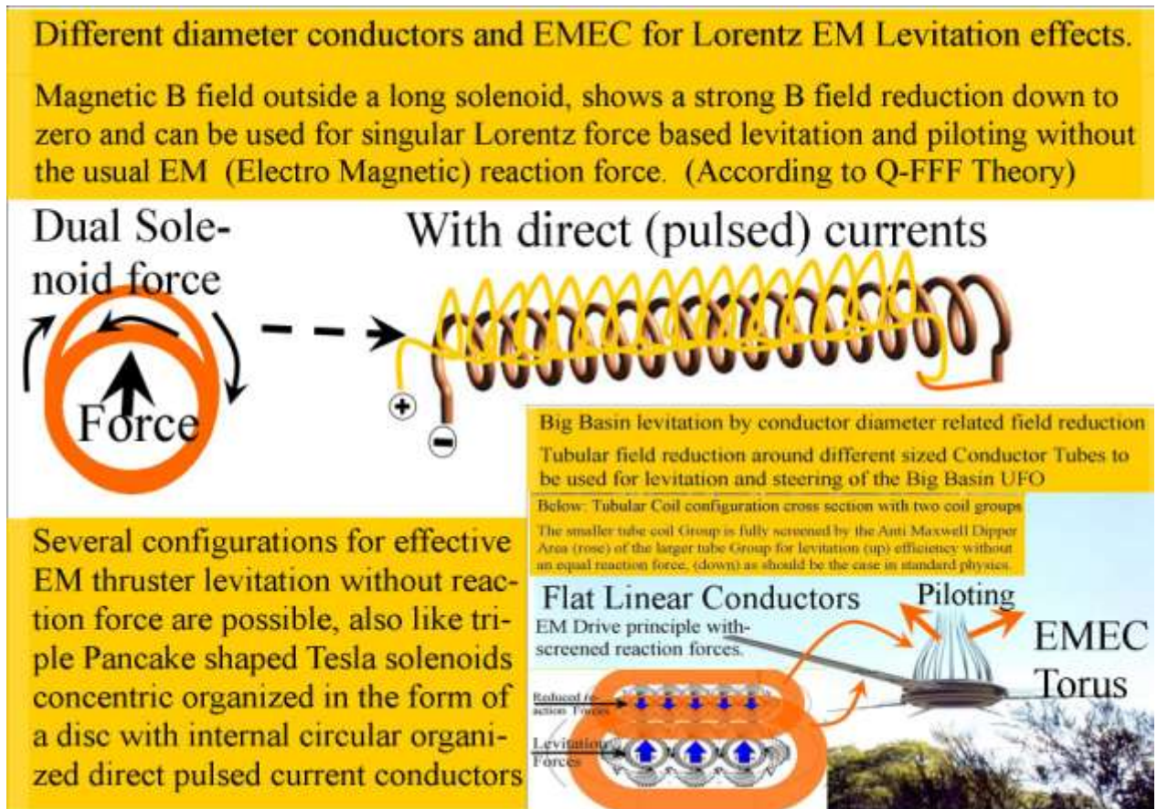
Figure 5. Levitation by different conductor diameter creating resistance less Lorentz force.
