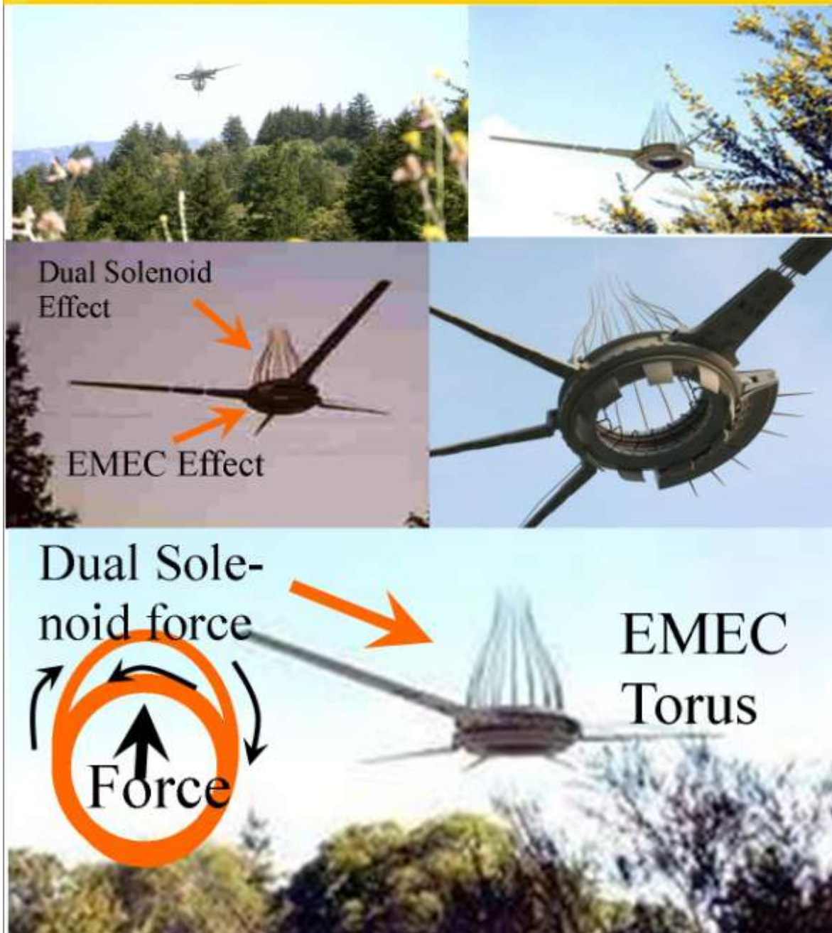
Figure 4. Some Big Basin examples with EMEC and Dual solenoidal Lorentz force.
