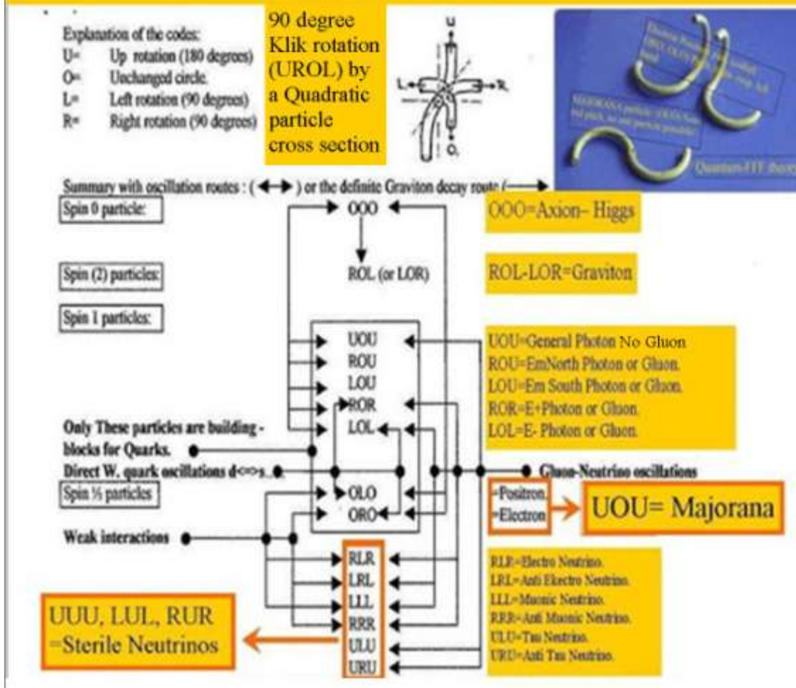
Figure 9, Overview String Transformation possibilities of Q-FFF Theory.
