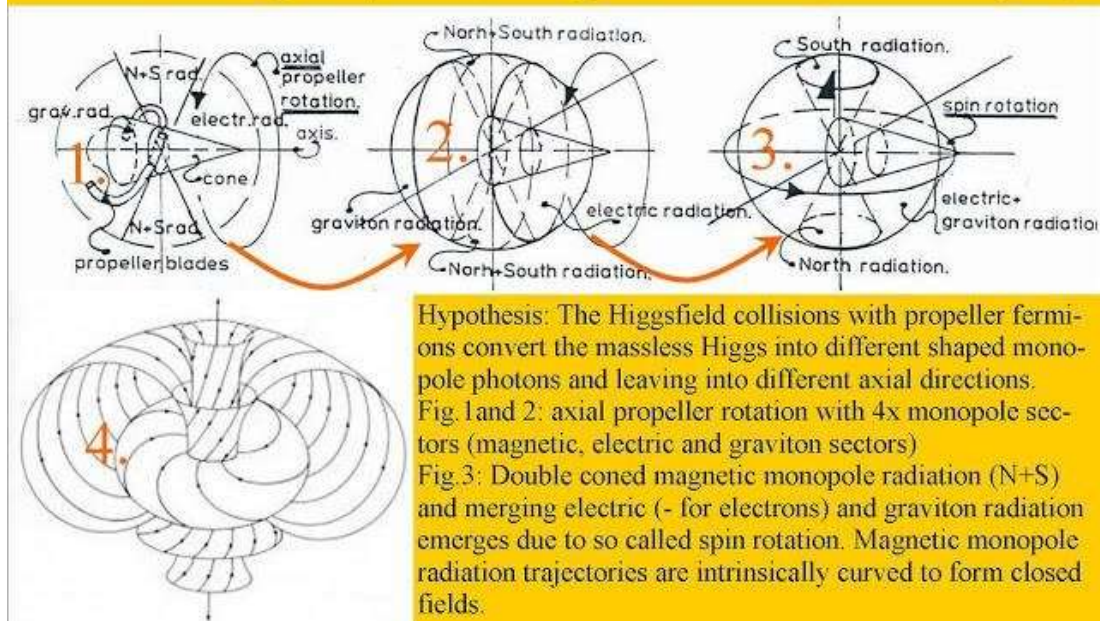
Figure 11, dual rotation of Leptons and Quarks.
