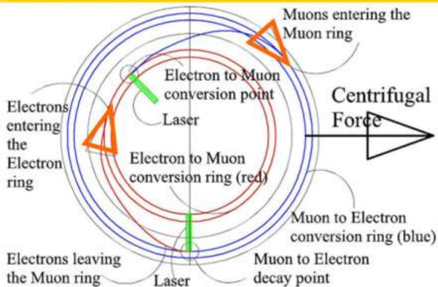
Figure 1, Overview of the dual concentric EMEC centrifugal Force creating rotation tubes.
