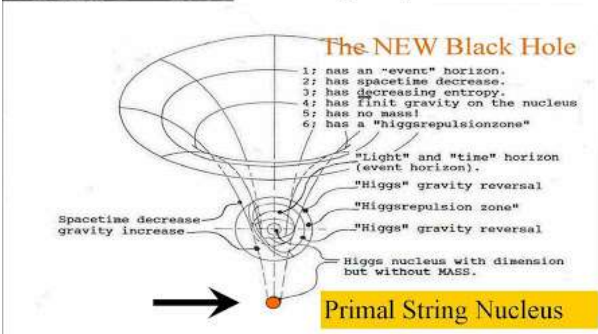
Figure 14, The new black hole.
