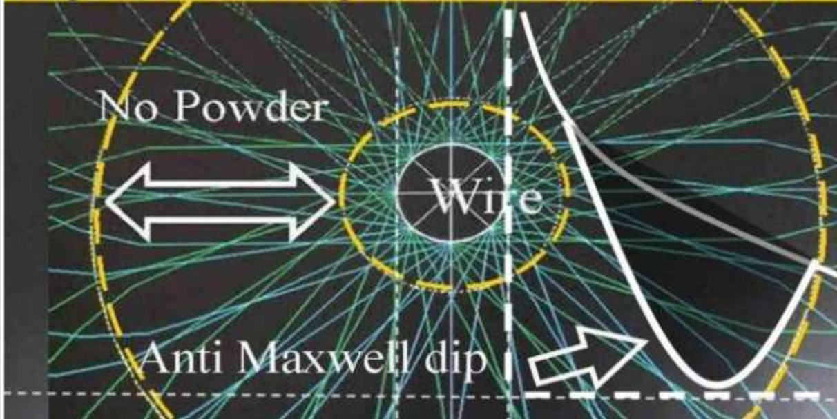
Figure 7, Triple Tesla Pancake coil with different diameter conductors.
