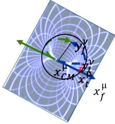
Figure 4: The contribution of \mathcal{P}I_{B_{active}(for: x_{CM}^\mu, t)}(S, \psi) |_{(part(t) \in D(M))} includes integration over 2\pi . The bundles of fold are sets of tori. Here, we assume: D(M) = [x_{CM(t)}^\mu, x_t^\mu(part_1)] \cup [x_{CM(t)}^\mu, x_t^\mu(part_2)] .
