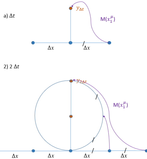
Figure 14: Growth of entangled spacetime by random walk or at inflation has spacetime points entangled locally at least for a while. The growth in spacetime matches the growth of the multi-folds. These deltas in spacetime and in folds are the quantas of the multi-fold mechanism (growth of the multi-folds), on in each fold, per (random) time click. They match the space-time growth or changes in \mathcal{R}_{BG} encountered in conventional quantization of gravity / GR and of gravity as a result. These are the gravitons in \mathcal{U}_{MF} : in our model, they live outside the spacetime \mathcal{R}_{BG} but match the perturbation and growth in \mathcal{R}_{BG} .
