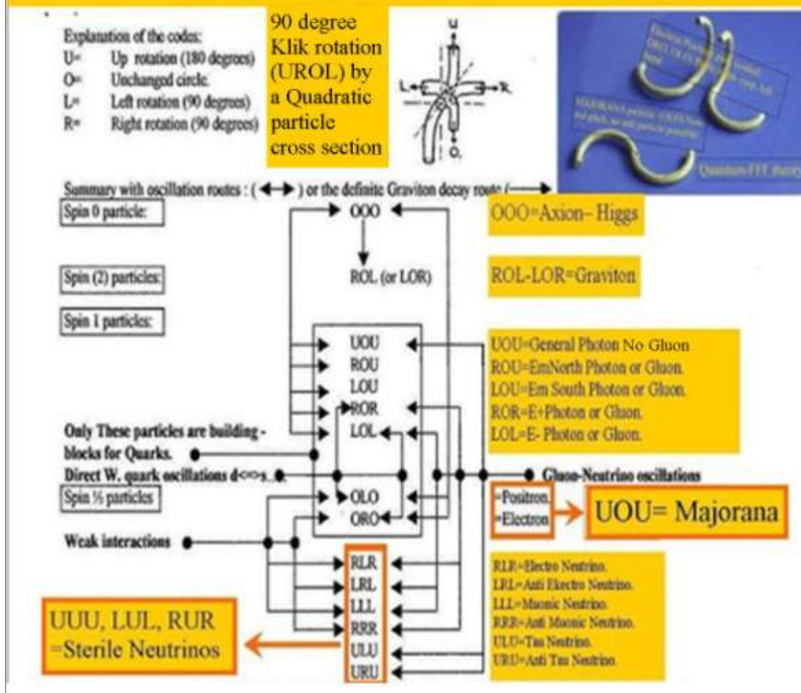
Figure 5, Overview String Transformation possibilities of Q-FFF Theory.
