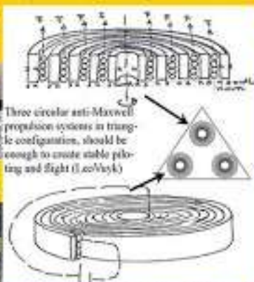
Several observations and explanation by the curvature of monopole quantum information arrays.
