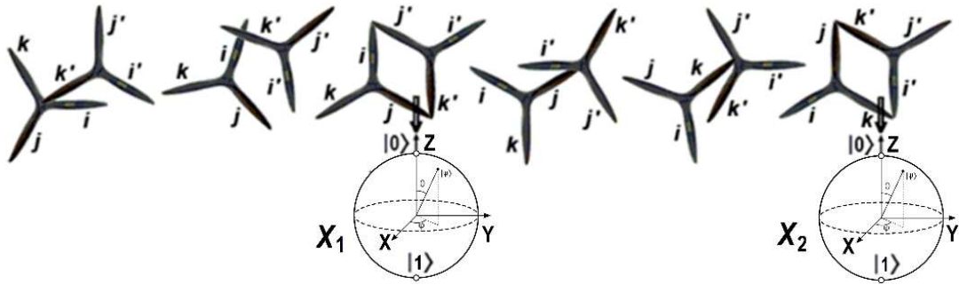
Figure 1. Spacetime, Space – Antispace duality. Points X_1 and X_2 represent infinitesimally separated Bloch 2-spheres (quantum bits) in spacetime. The six mirror symmetric i,j,k pairs exist in HD space hidden from observation by the uncertainty principle.
