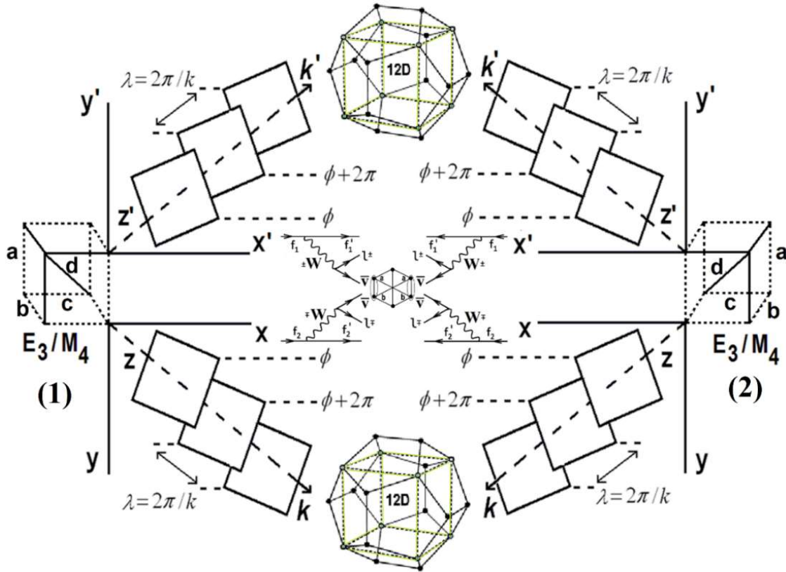
Figure 5. Calabi-Yau future-past mirror symmetry potential dual 3-tori illustrated as tiered surfaces of constant phase, in this case to represent cyclic components evenly spaced orthogonal standing reality waves with the E_3/M_4 cubic (3-space) resultant line element points in t , localized left, x_1 and right, x_2 . We do not know how to draw this yet; the center represents the 12D LSXD superspace causally-free copy of the local quantum state in 3-space.
