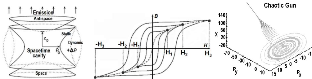
Figure 7. a) Model of spacetime MOU QED cavity as a static-dynamic Casimir of UFM charge. The cavity opens and closes; timing is crucial. b) Charge characteristics of nested Hysteresis loops used for modeling the cyclic cavity dynamics of fermionic space-antispacetime parameters. Our postulate is that the Dirac polarized vacuum can demonstrate hysteresis properties. c) Simplistic summation of UFM coherence for DEB operation.
