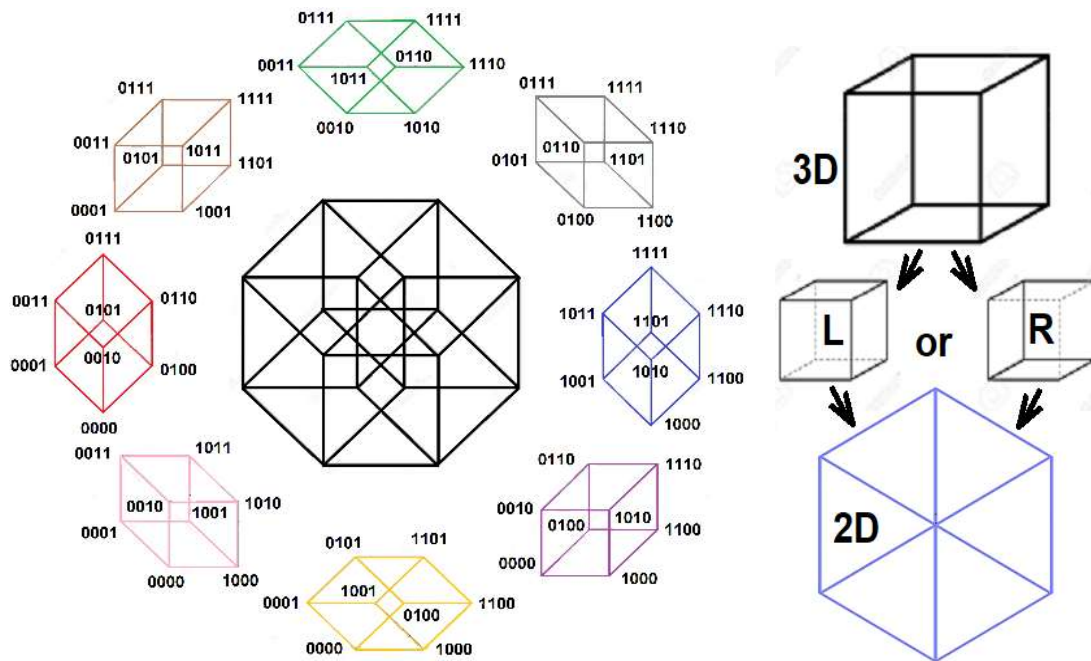
Figure 4. a) Exploded 4D hypercube, 64 overlapping vertices (4) or 16 subsets ( 16 \times 4 = 64 ). One of four orthogonal configurations, with mirror symmetry another four. In terms of developing the required UFM transform, each 3-cube represents an ambiguous Necker (b) cube able to perform topological raising and lowering moves. The four cubes illustrated have interplaying vertex points, dotted – 0101:1011 and 0100:1010; solid – 0110:1101 and 0010:1001. b-bottom) Conceptualized view of the HD quadrupole photon-vacuum complex for quadrupole \leftrightarrow dipole interactions as elements of the U_F at the event horizon of Minkowski spacetime. b) Dimensional reduction.
