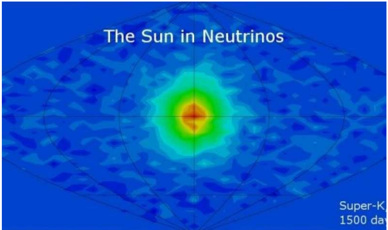
A graphic showing neutrinos emitted from the sun over a period of 1500 days. Credit: T2K Experiment
