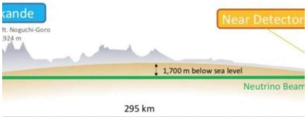
Diagram of how the T2K experiment sends and detects beams of neutrinos. Credits: T2K Experiment
