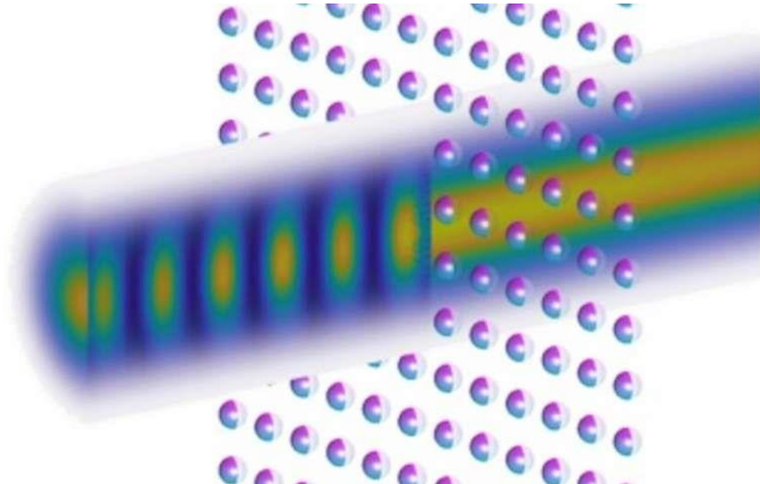
A schematic figure of scattering from the quantum metasurface in a superposition state. Credit: Bekenstein et al.
