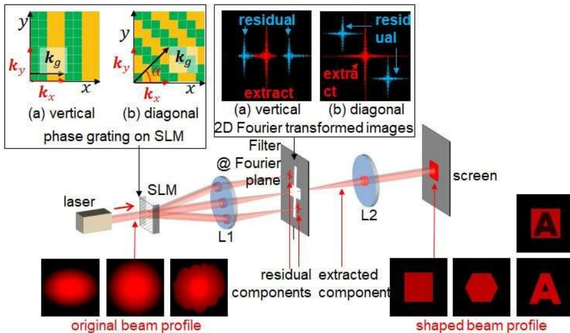
Figure 2. Experimental layout: phase grating and filtering in the Fourier plane of the 4f system.
