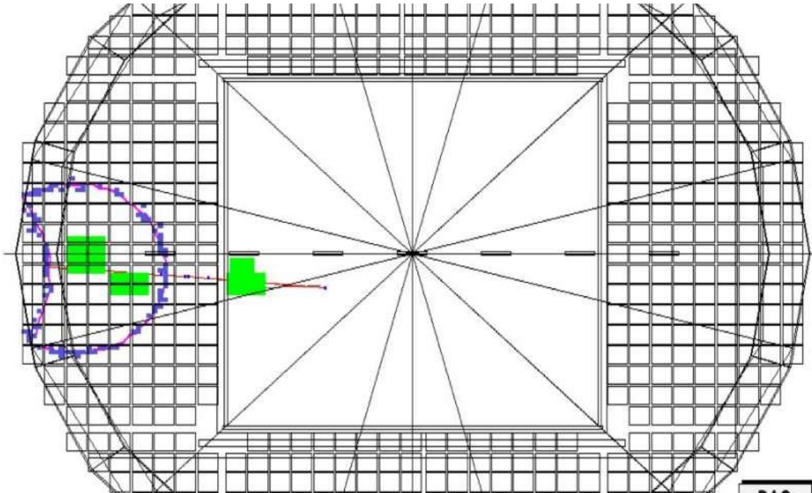
An event display of the signal that can be reconstructed by the RICH detector. Credit: CERN.
