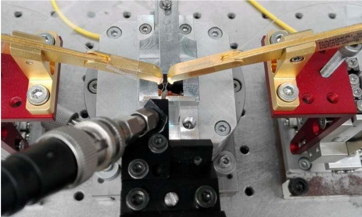
Experimental setup used to characterise a prototype of the novel light detector. Credit: ETH Zurich
