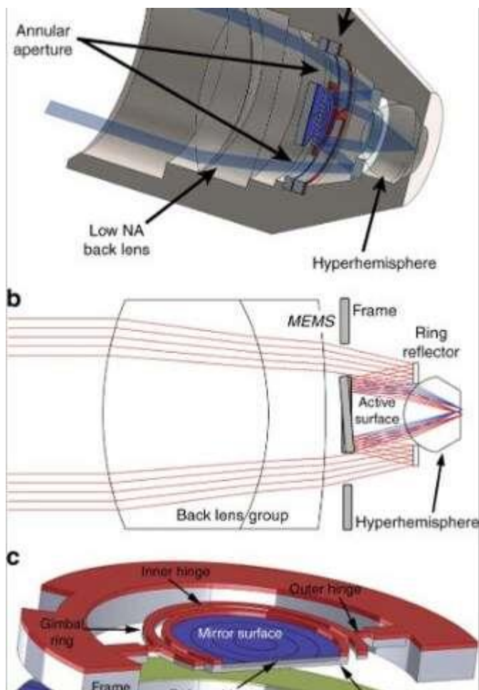
MEMS-in-the-lens architecture. (a) A cross-sectional view of the miniaturized confocal microscope with a new objective lens that incorporates a MEMS 3D scanner. (b) An illustration of the light path through the annular aperture and the beam scan of the MEMS device. (c) A model of the MEMS 3D scanner. A gimbal platform is bonded to a set of quadrant electrodes. Credit: Light: Science & Applications , doi: 10.1038/s41377-019-0167-5
