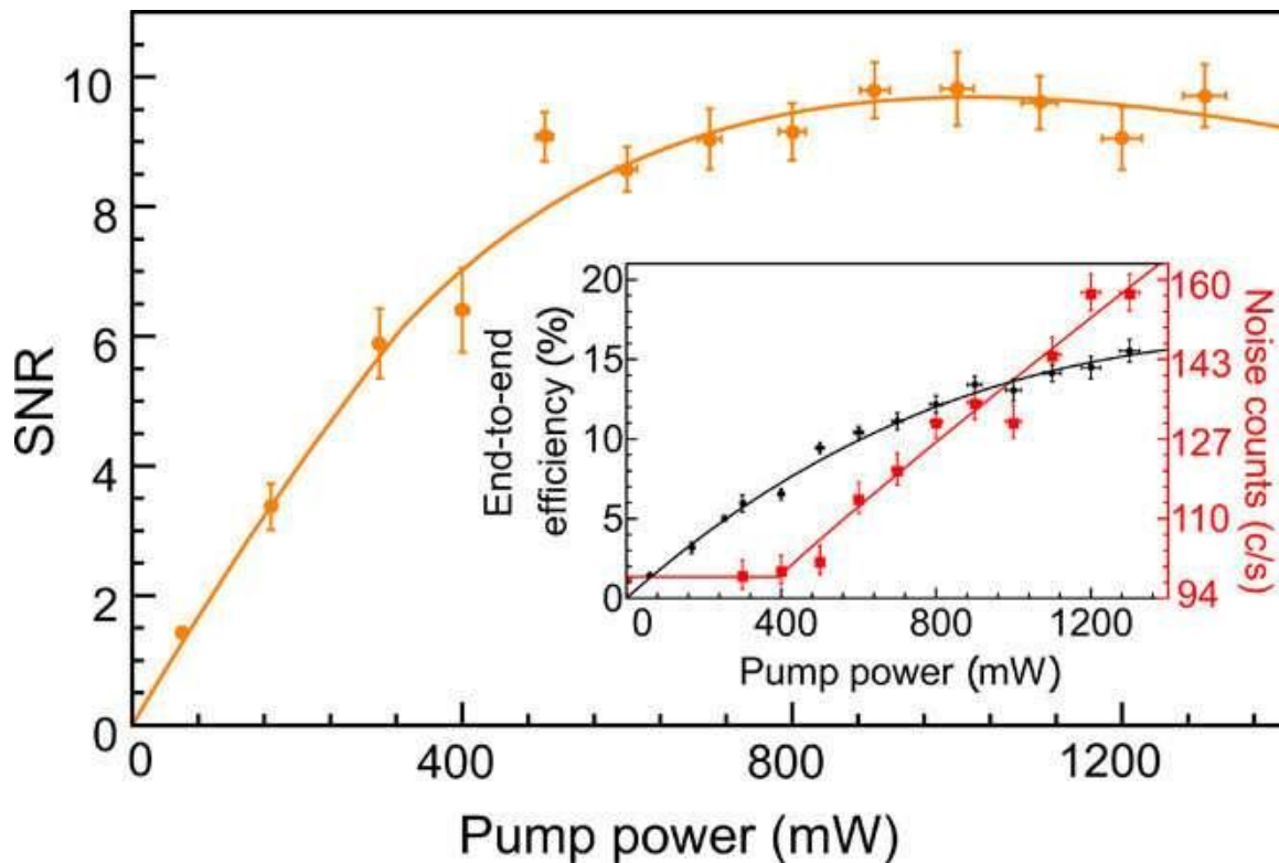
Signal-to-noise-ratio (SNR) measured after filtering of the frequency-converted ion signal. The
