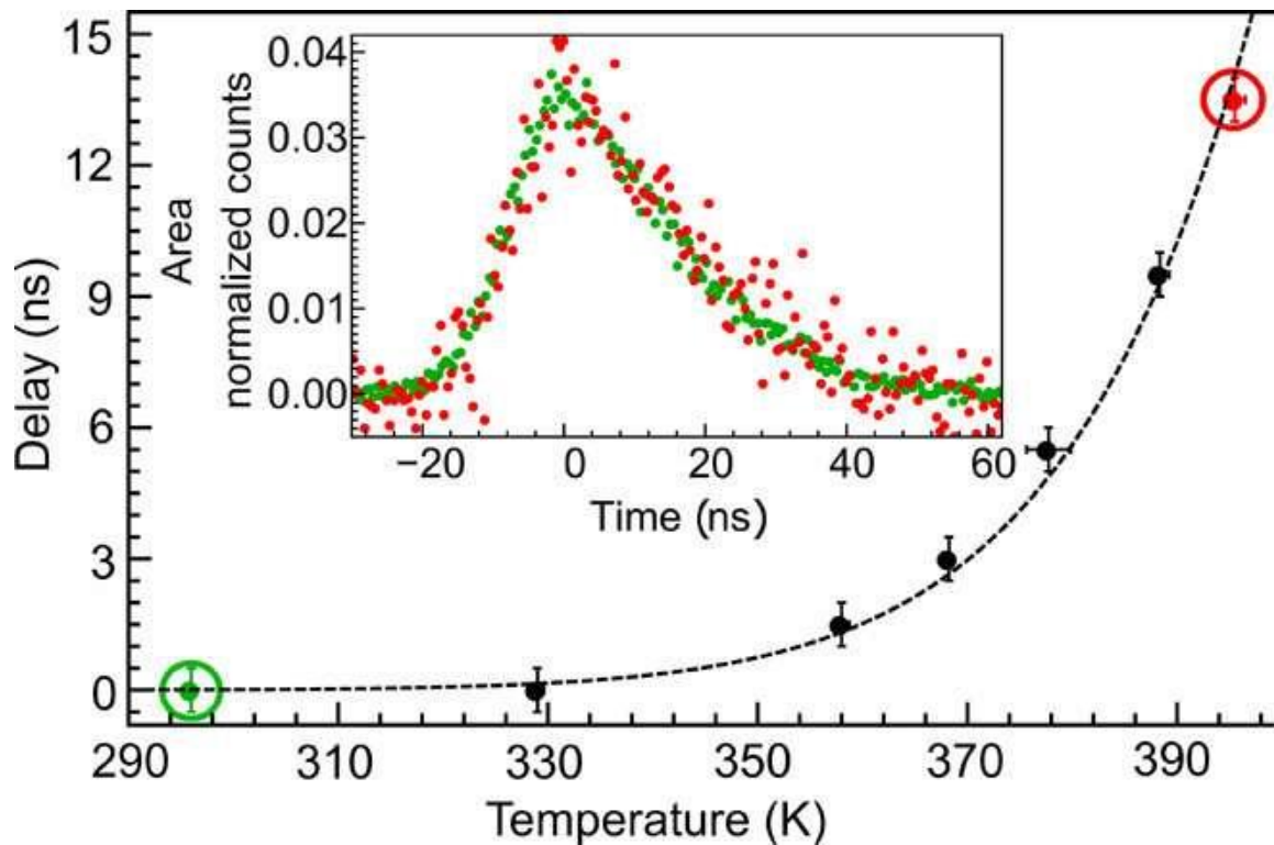
Delay of the frequency-converted photons emitted from the trapped \text{Ba}^+ ion after passing through a ^{87}\text{Rb} vapor cell as a function of the cell's temperature. The dashed theory curve is a scaled version of the equation derived in the work to account for N . The temperature and delay error bars
