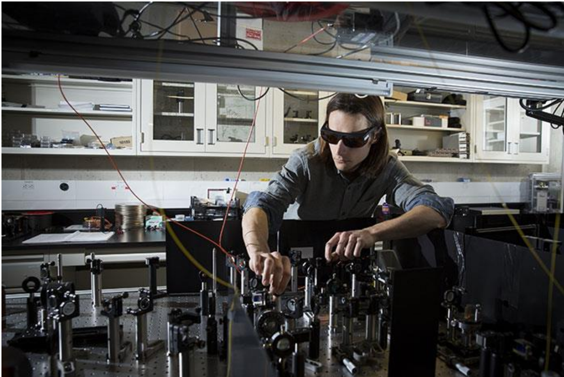
Energy-time entanglement detected in photons
