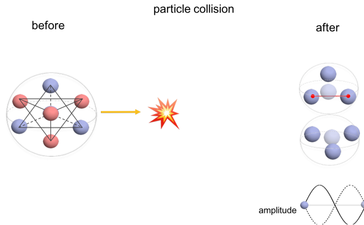
Fig. 3.7 – A particle colliding with other particles may rearrange wave centers and become two or more particles
