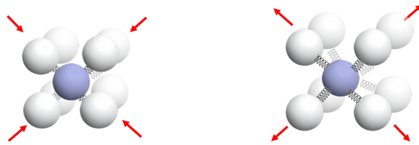
Fig. 1.2 – Wave center (blue)
