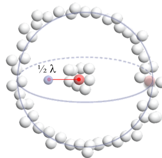
Fig. 2.2 – The antiparticle results from a wave center (center in red) that is at the opposite node ( 1/2 \lambda ).
