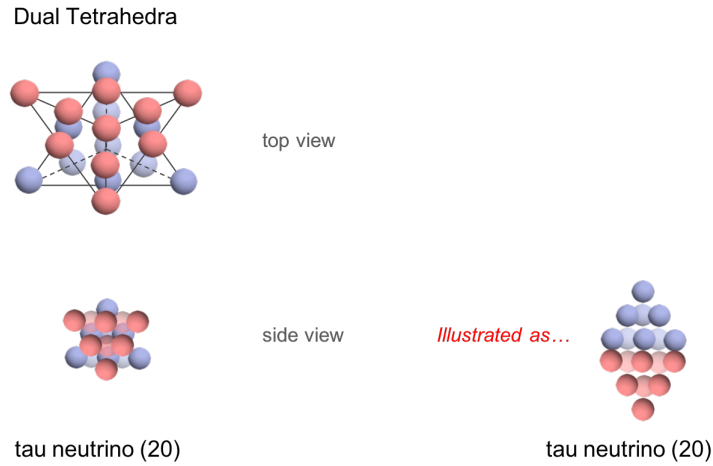
Fig. 5.2 – Particles may form dual tetrahedra as illustrated for the tau neutrino. Due to the complexity viewing dual tetrahedra, it is illustrated as two symmetrical tetrahedra in the figure (illustration on the right in Fig. 5.2).
