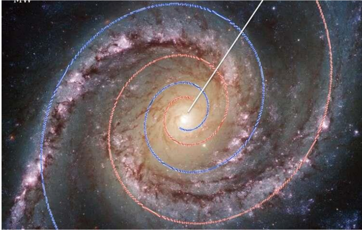
A spiral galaxy with an overlaid double-armed logarithmic spiral. Credit: Parker & Jaynes, Fig.2 of Scientific Reports 9|10779 (2019), CC BY-SA
