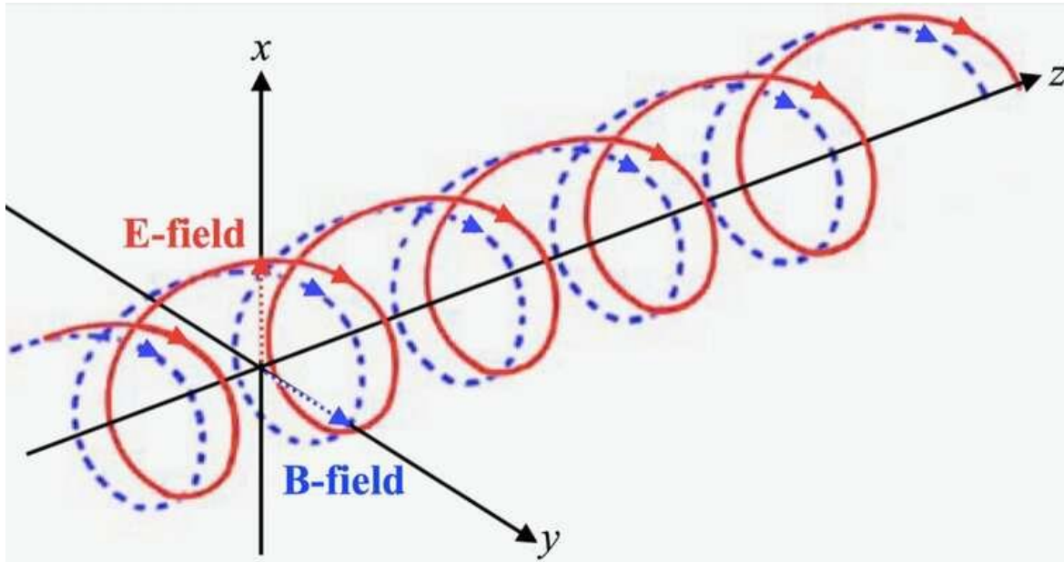
Light wave with electric (E) and magnetic (B) fields. Author provided
